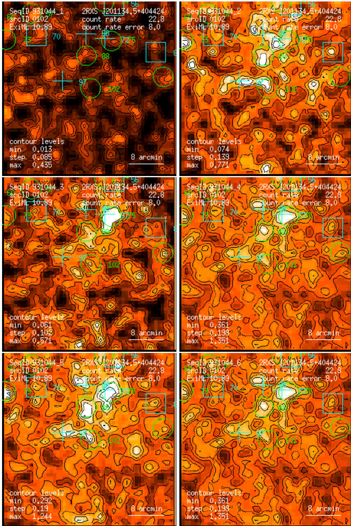
Figure 102: RASS 931044: detection 0102: band rate images, Gaussian filter: (1) PSPC channels 11 – 41, (2) 52 – 90, (3) 91 – 201, (4) 11 – 235, (5) 52 – 201, (6) 11 – 201. Broad band rates in counts/ks. Band rate contour levels in counts/ks/arcmin 2 .
