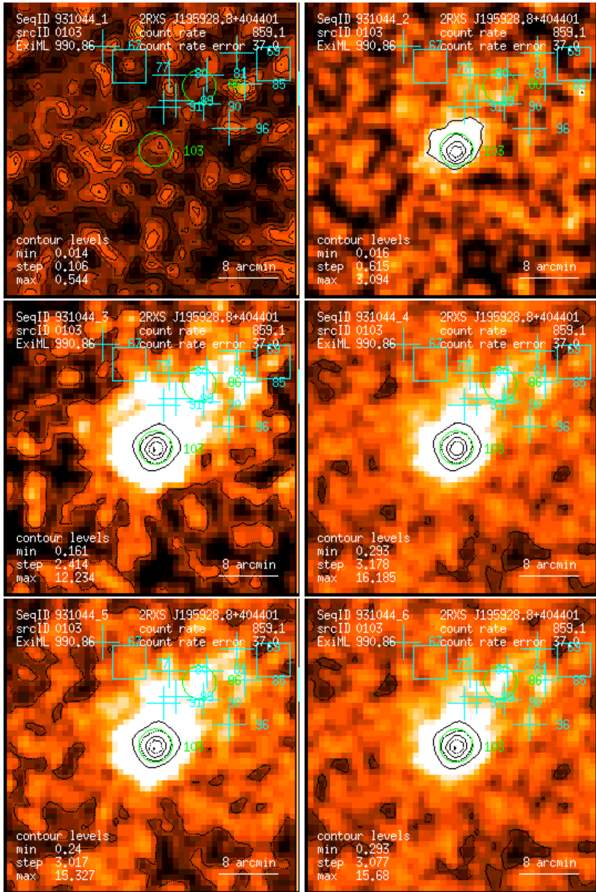
Figure 103: RASS 931044: detection 0103: band rate images, Gaussian filter: (1) PSPC channels 11 – 41, (2) 52 – 90, (3) 91 – 201, (4) 11 – 235, (5) 52 – 201, (6) 11 – 201. Broad band rates in counts/ks. Band rate contour levels in counts/ks/arcmin 2 .
