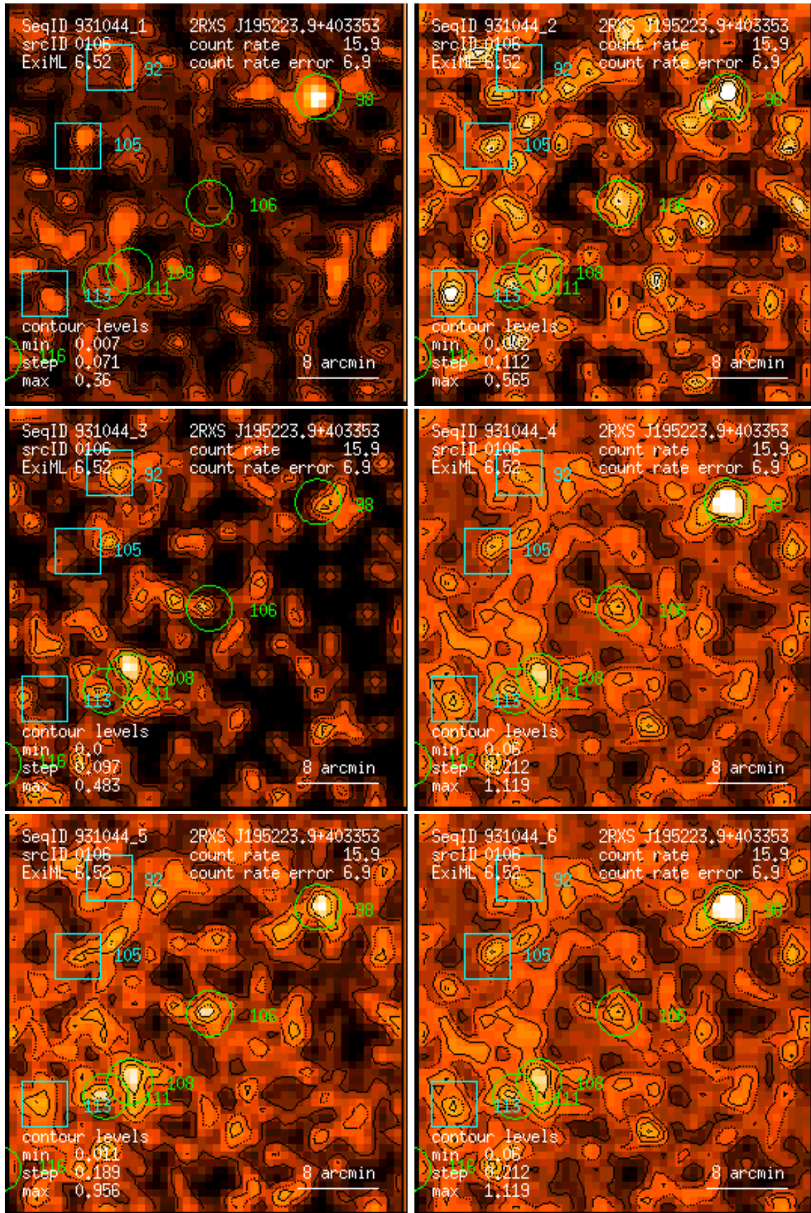
Figure 106: RASS 931044: detection 0106: band rate images, Gaussian filter: (1) PSPC channels 11 – 41, (2) 52 – 90, (3) 91 – 201, (4) 11 – 235, (5) 52 – 201, (6) 11 – 201. Broad band rates in counts/ks. Band rate contour levels in counts/ks/arcmin 2 .
