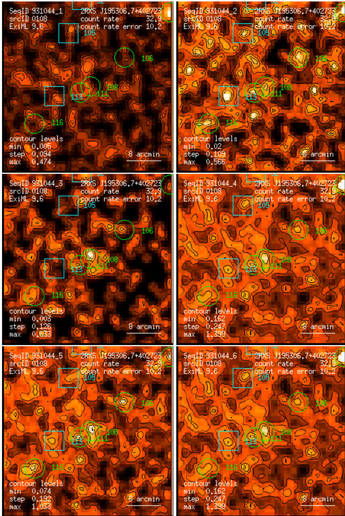
Figure 108: RASS 931044: detection 0108: band rate images, Gaussian filter: (1) PSPC channels 11 – 41, (2) 52 – 90, (3) 91 – 201, (4) 11 – 235, (5) 52 – 201, (6) 11 – 201. Broad band rates in counts/ks. Band rate contour levels in counts/ks/arcmin 2 .
