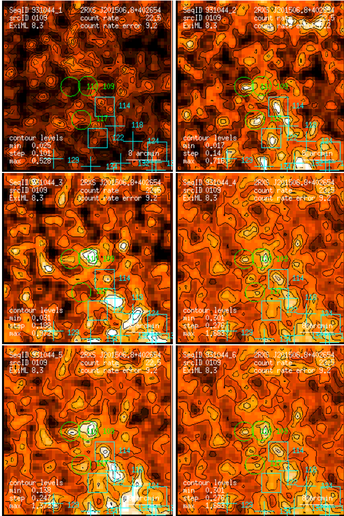
Figure 109: RASS 931044: detection 0109: band rate images, Gaussian filter: (1) PSPC channels 11 – 41, (2) 52 – 90, (3) 91 – 201, (4) 11 – 235, (5) 52 – 201, (6) 11 – 201. Broad band rates in counts/ks. Band rate contour levels in counts/ks/arcmin 2 .
