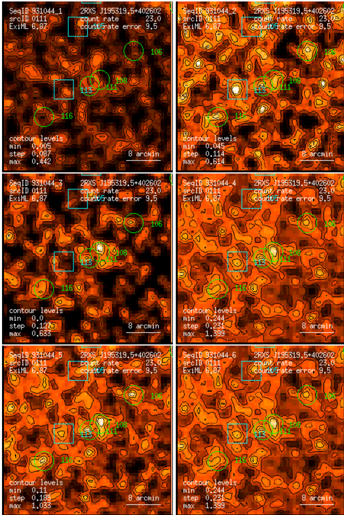
Figure 111: RASS 931044: detection 0111: band rate images, Gaussian filter: (1) PSPC channels 11 – 41, (2) 52 – 90, (3) 91 – 201, (4) 11 – 235, (5) 52 – 201, (6) 11 – 201. Broad band rates in counts/ks. Band rate contour levels in counts/ks/arcmin 2 .
