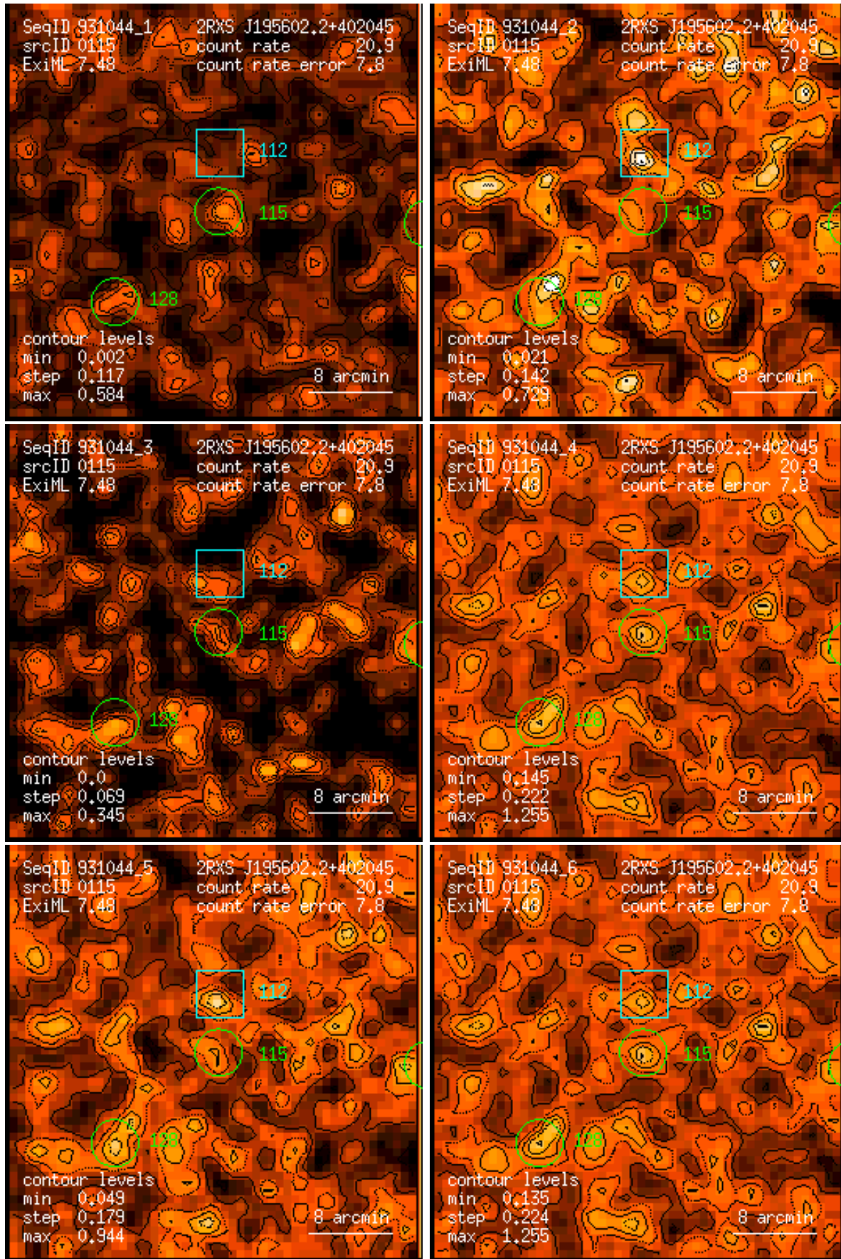
Figure 115: RASS 931044: detection 0115: band rate images, Gaussian filter: (1) PSPC channels 11 – 41, (2) 52 – 90, (3) 91 – 201, (4) 11 – 235, (5) 52 – 201, (6) 11 – 201. Broad band rates in counts/ks. Band rate contour levels in counts/ks/arcmin 2 .
