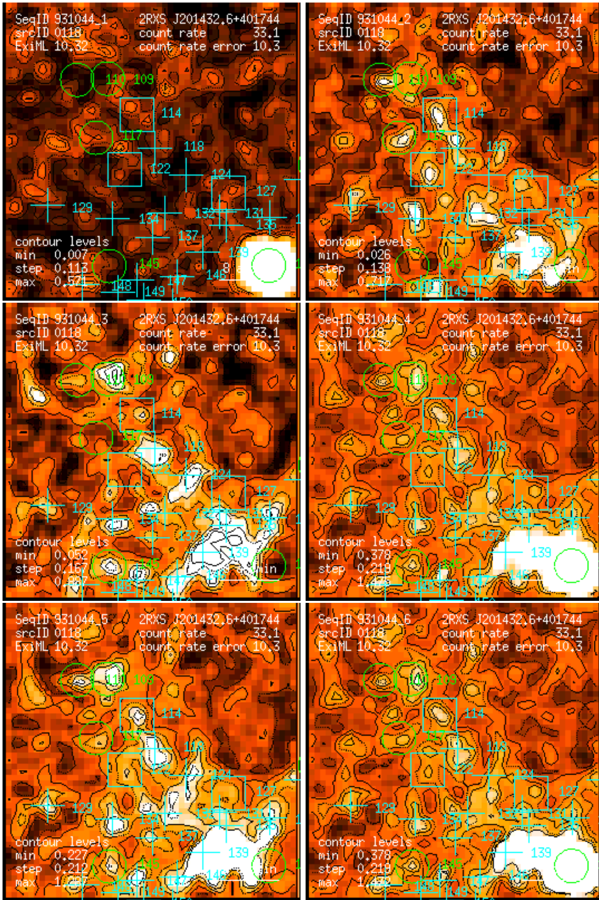
Figure 118: RASS 931044: detection 0118: band rate images, Gaussian filter: (1) PSPC channels 11 – 41, (2) 52 – 90, (3) 91 – 201, (4) 11 – 235, (5) 52 – 201, (6) 11 – 201. Broad band rates in counts/ks. Band rate contour levels in counts/ks/arcmin 2 .
