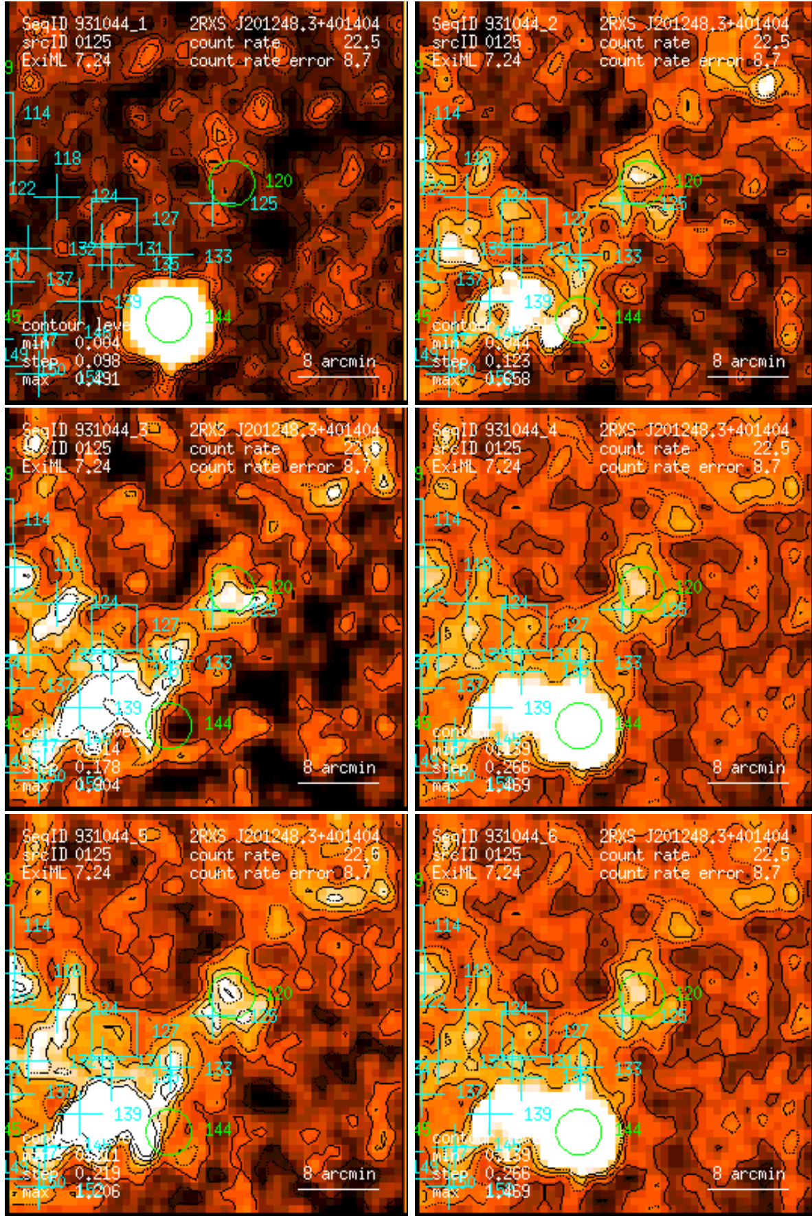
Figure 125: RASS 931044: detection 0125: band rate images, Gaussian filter: (1) PSPC channels 11 – 41, (2) 52 – 90, (3) 91 – 201, (4) 11 – 235, (5) 52 – 201, (6) 11 – 201. Broad band rates in counts/ks. Band rate contour levels in counts/ks/arcmin 2 .
