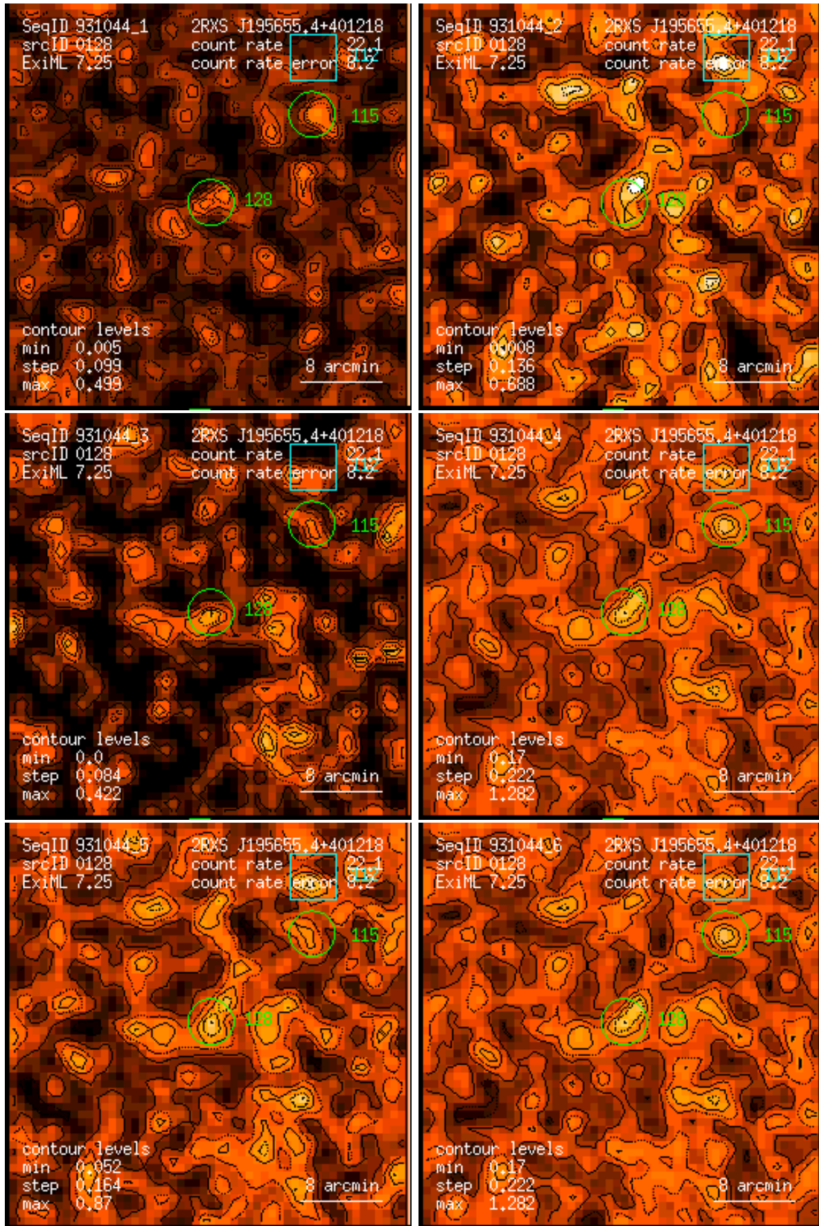
Figure 128: RASS 931044: detection 0128: band rate images, Gaussian filter: (1) PSPC channels 11 – 41, (2) 52 – 90, (3) 91 – 201, (4) 11 – 235, (5) 52 – 201, (6) 11 – 201. Broad band rates in counts/ks. Band rate contour levels in counts/ks/arcmin 2 .
