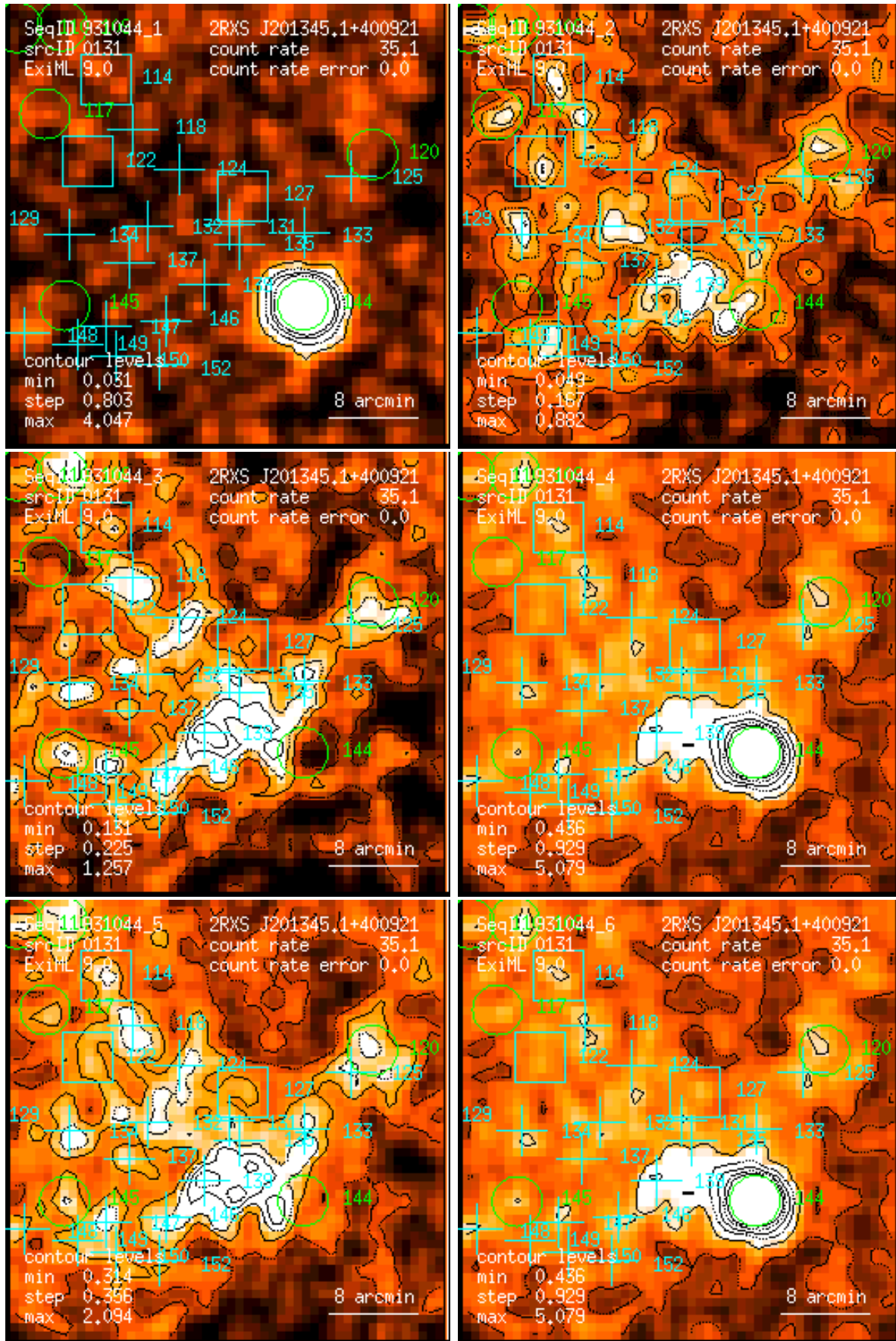
Figure 131: RASS 931044: detection 0131: band rate images, Gaussian filter: (1) PSPC channels 11 – 41, (2) 52 – 90, (3) 91 – 201, (4) 11 – 235, (5) 52 – 201, (6) 11 – 201. Broad band rates in counts/ks. Band rate contour levels in counts/ks/arcmin 2 .
