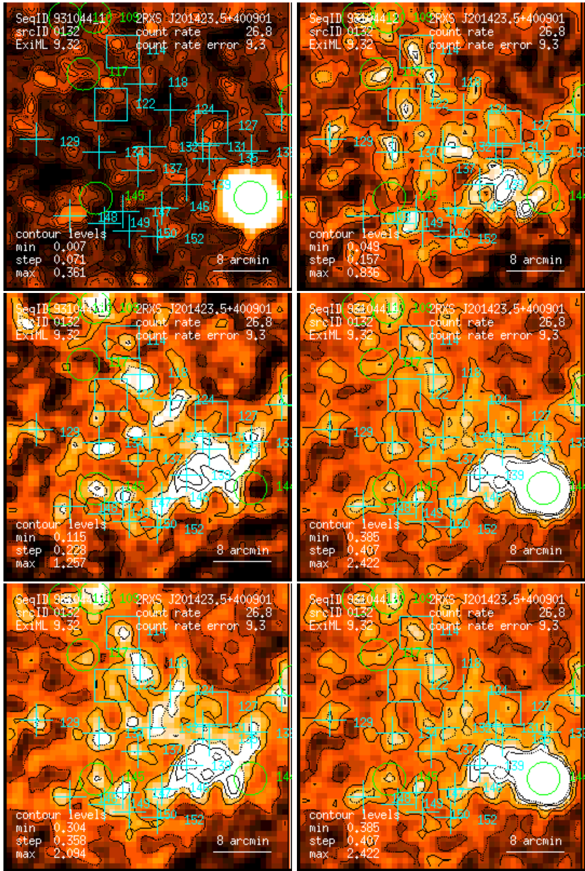
Figure 132: RASS 931044: detection 0132: band rate images, Gaussian filter: (1) PSPC channels 11 – 41, (2) 52 – 90, (3) 91 – 201, (4) 11 – 235, (5) 52 – 201, (6) 11 – 201. Broad band rates in counts/ks. Band rate contour levels in counts/ks/arcmin 2 .
