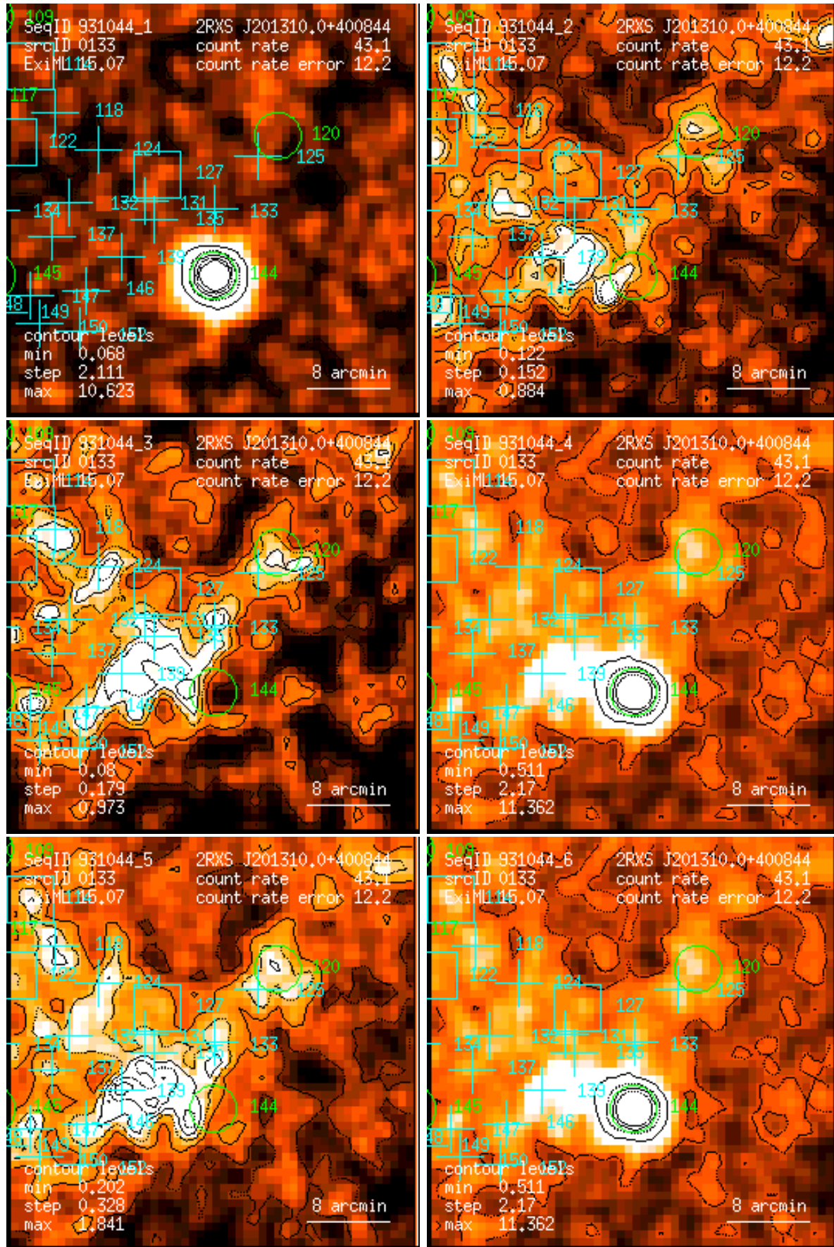
Figure 133: RASS 931044: detection 0133: band rate images, Gaussian filter: (1) PSPC channels 11 – 41, (2) 52 – 90, (3) 91 – 201, (4) 11 – 235, (5) 52 – 201, (6) 11 – 201. Broad band rates in counts/ks. Band rate contour levels in counts/ks/arcmin 2 .
