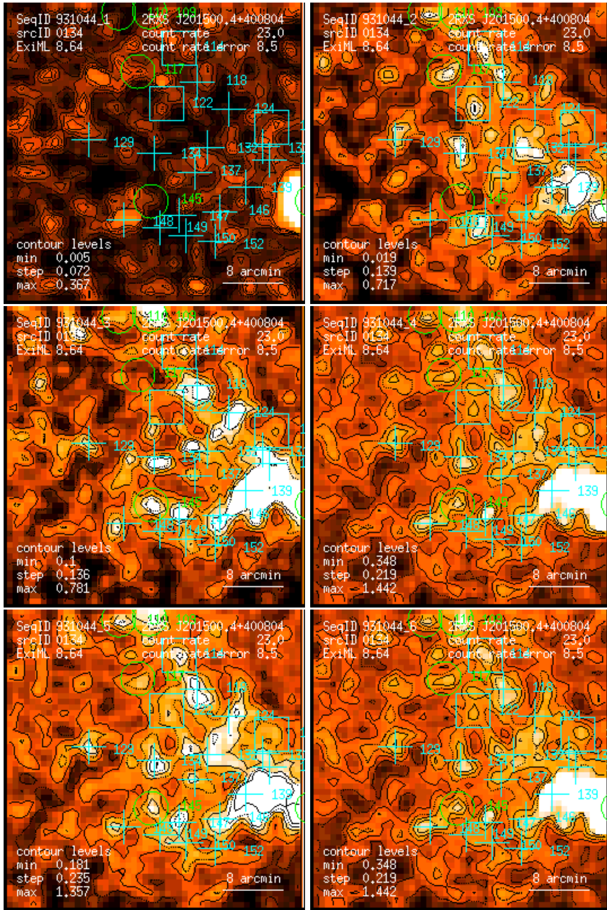
Figure 134: RASS 931044: detection 0134: band rate images, Gaussian filter: (1) PSPC channels 11 – 41, (2) 52 – 90, (3) 91 – 201, (4) 11 – 235, (5) 52 – 201, (6) 11 – 201. Broad band rates in counts/ks. Band rate contour levels in counts/ks/arcmin 2 .
