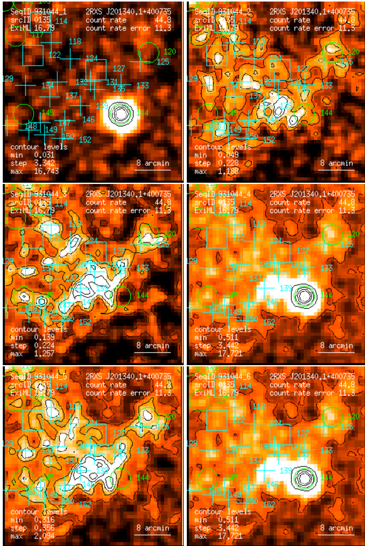
Figure 135: RASS 931044: detection 0135: band rate images, Gaussian filter: (1) PSPC channels 11 – 41, (2) 52 – 90, (3) 91 – 201, (4) 11 – 235, (5) 52 – 201, (6) 11 – 201. Broad band rates in counts/ks. Band rate contour levels in counts/ks/arcmin 2 .
