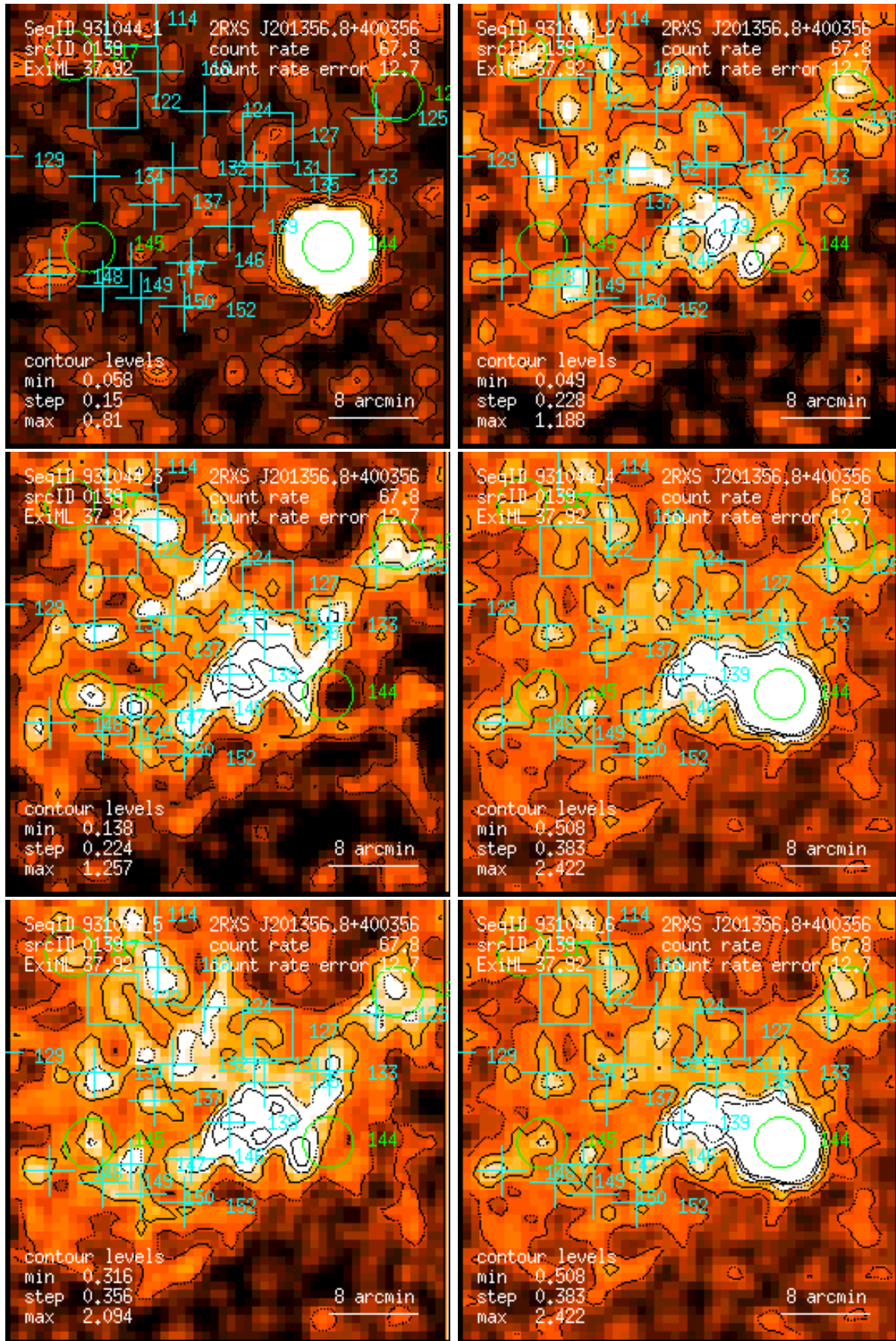
Figure 139: RASS 931044: detection 0139: band rate images, Gaussian filter: (1) PSPC channels 11 – 41, (2) 52 – 90, (3) 91 – 201, (4) 11 – 235, (5) 52 – 201, (6) 11 – 201. Broad band rates in counts/ks. Band rate contour levels in counts/ks/arcmin 2 .
