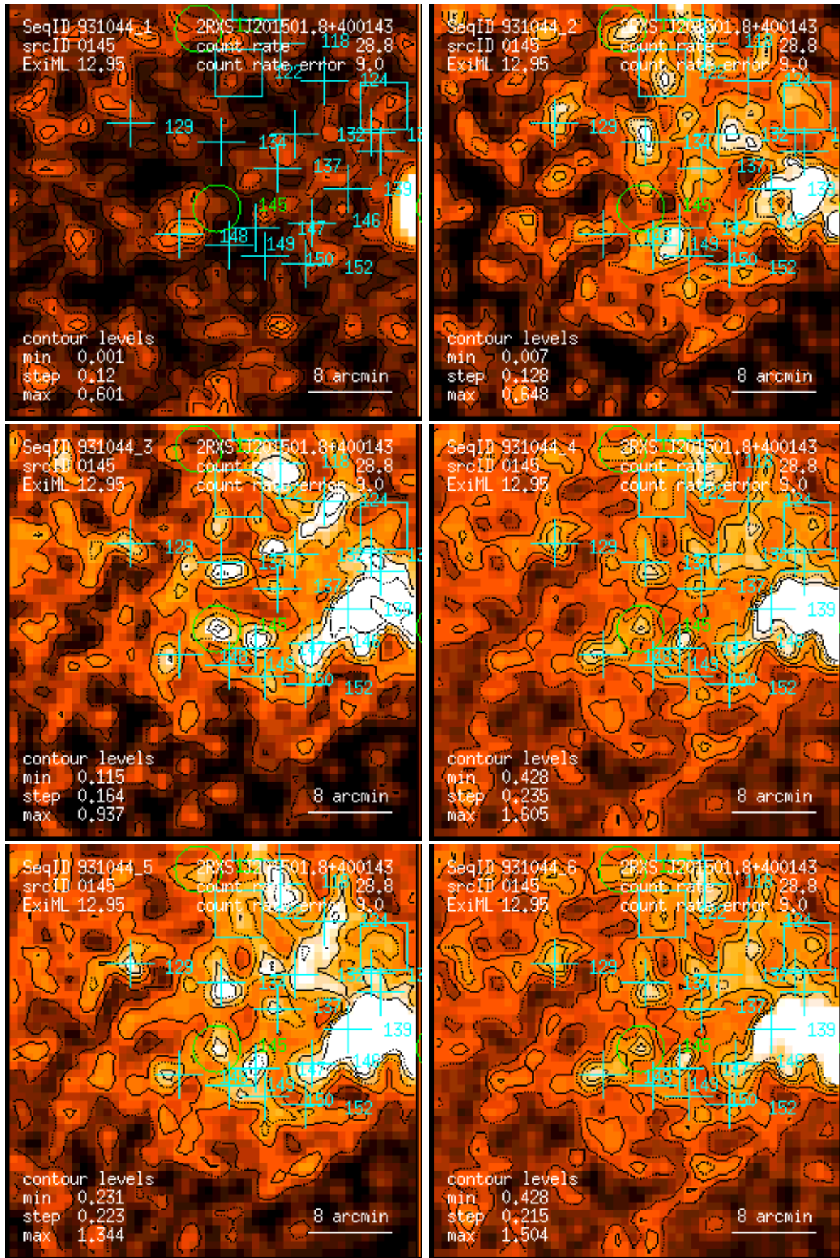
Figure 145: RASS 931044: detection 0145: band rate images, Gaussian filter: (1) PSPC channels 11 – 41, (2) 52 – 90, (3) 91 – 201, (4) 11 – 235, (5) 52 – 201, (6) 11 – 201. Broad band rates in counts/ks. Band rate contour levels in counts/ks/arcmin 2 .
