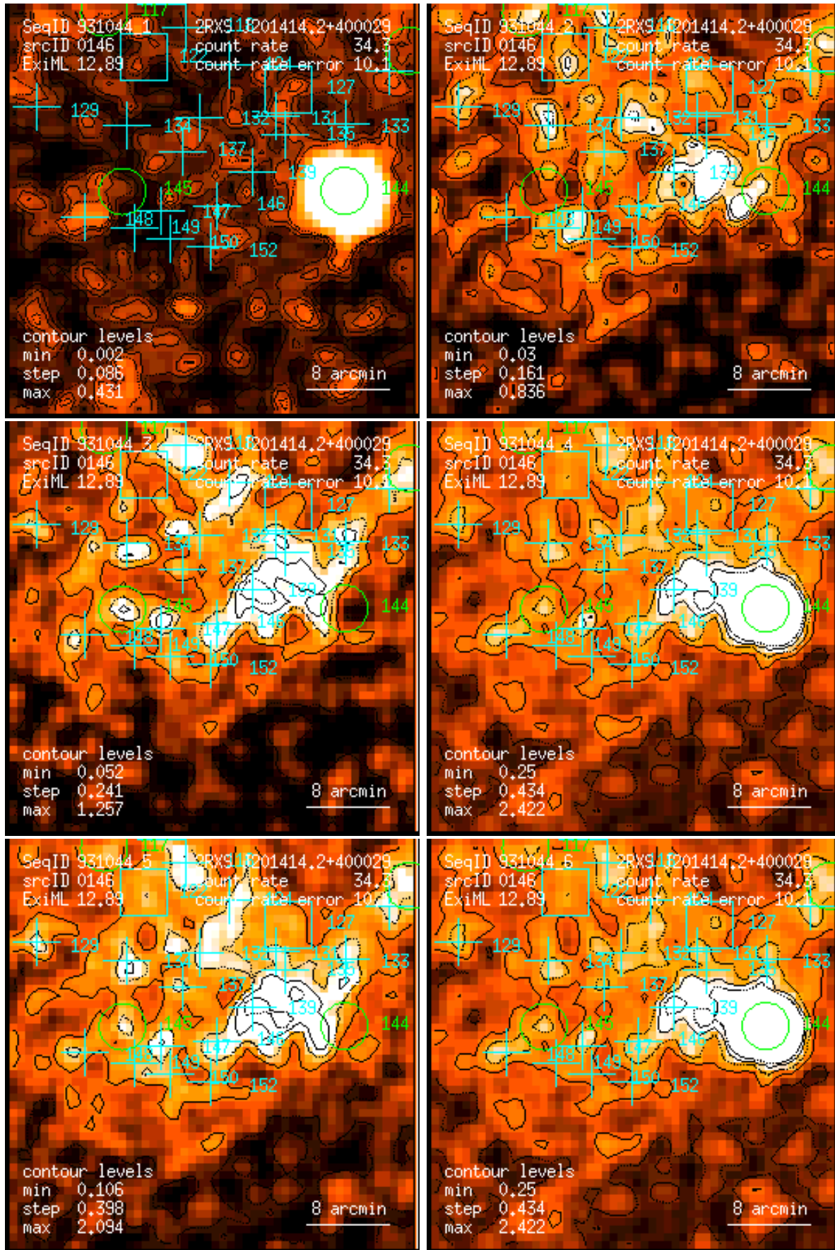
Figure 146: RASS 931044: detection 0146: band rate images, Gaussian filter: (1) PSPC channels 11 – 41, (2) 52 – 90, (3) 91 – 201, (4) 11 – 235, (5) 52 – 201, (6) 11 – 201. Broad band rates in counts/ks. Band rate contour levels in counts/ks/arcmin 2 .
