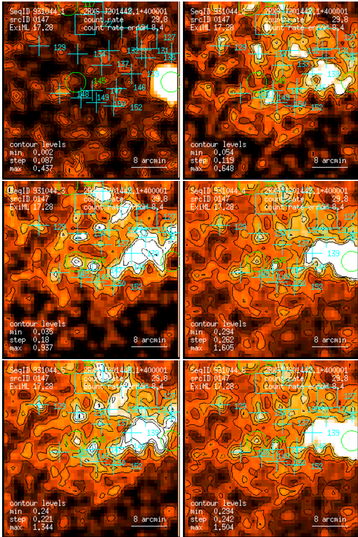
Figure 147: RASS 931044: detection 0147: band rate images, Gaussian filter: (1) PSPC channels 11 – 41, (2) 52 – 90, (3) 91 – 201, (4) 11 – 235, (5) 52 – 201, (6) 11 – 201. Broad band rates in counts/ks. Band rate contour levels in counts/ks/arcmin 2 .
