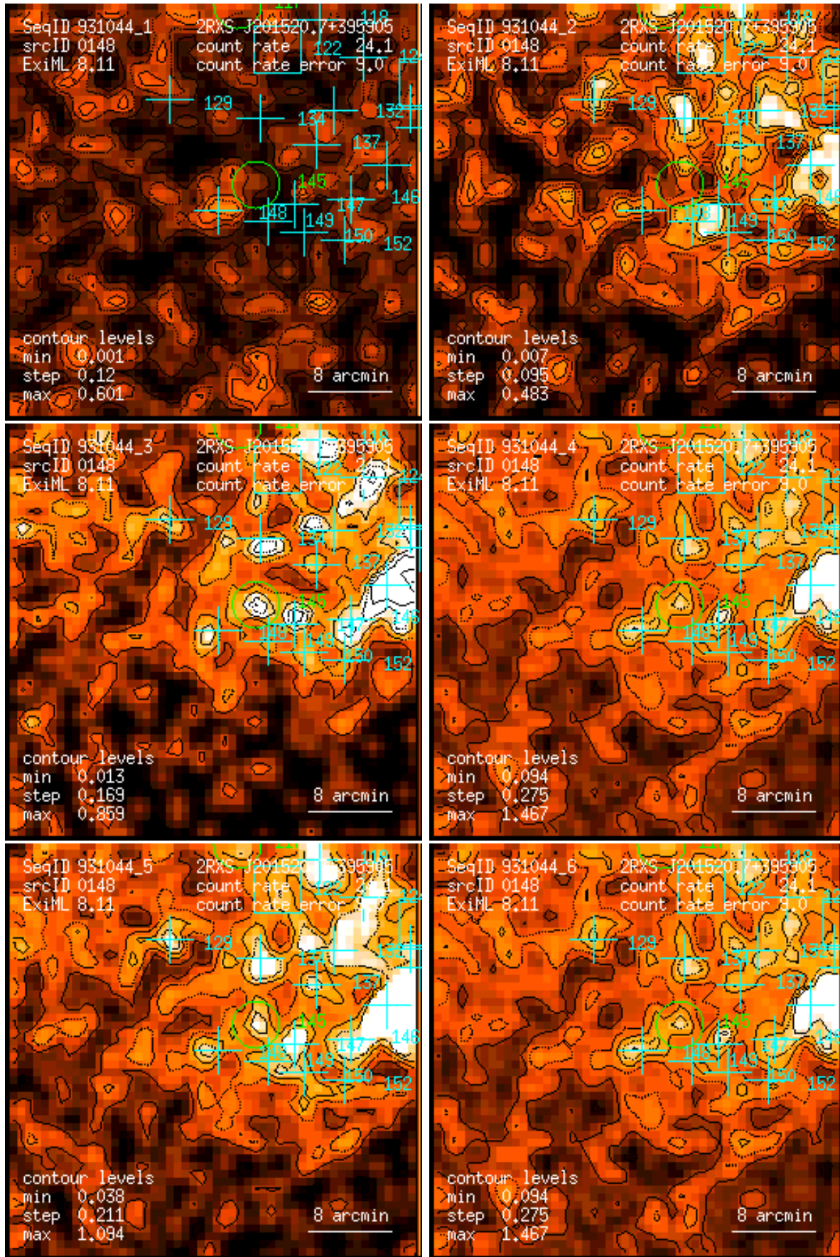
Figure 148: RASS 931044: detection 0148: band rate images, Gaussian filter: (1) PSPC channels 11 – 41, (2) 52 – 90, (3) 91 – 201, (4) 11 – 235, (5) 52 – 201, (6) 11 – 201. Broad band rates in counts/ks. Band rate contour levels in counts/ks/arcmin 2 .
