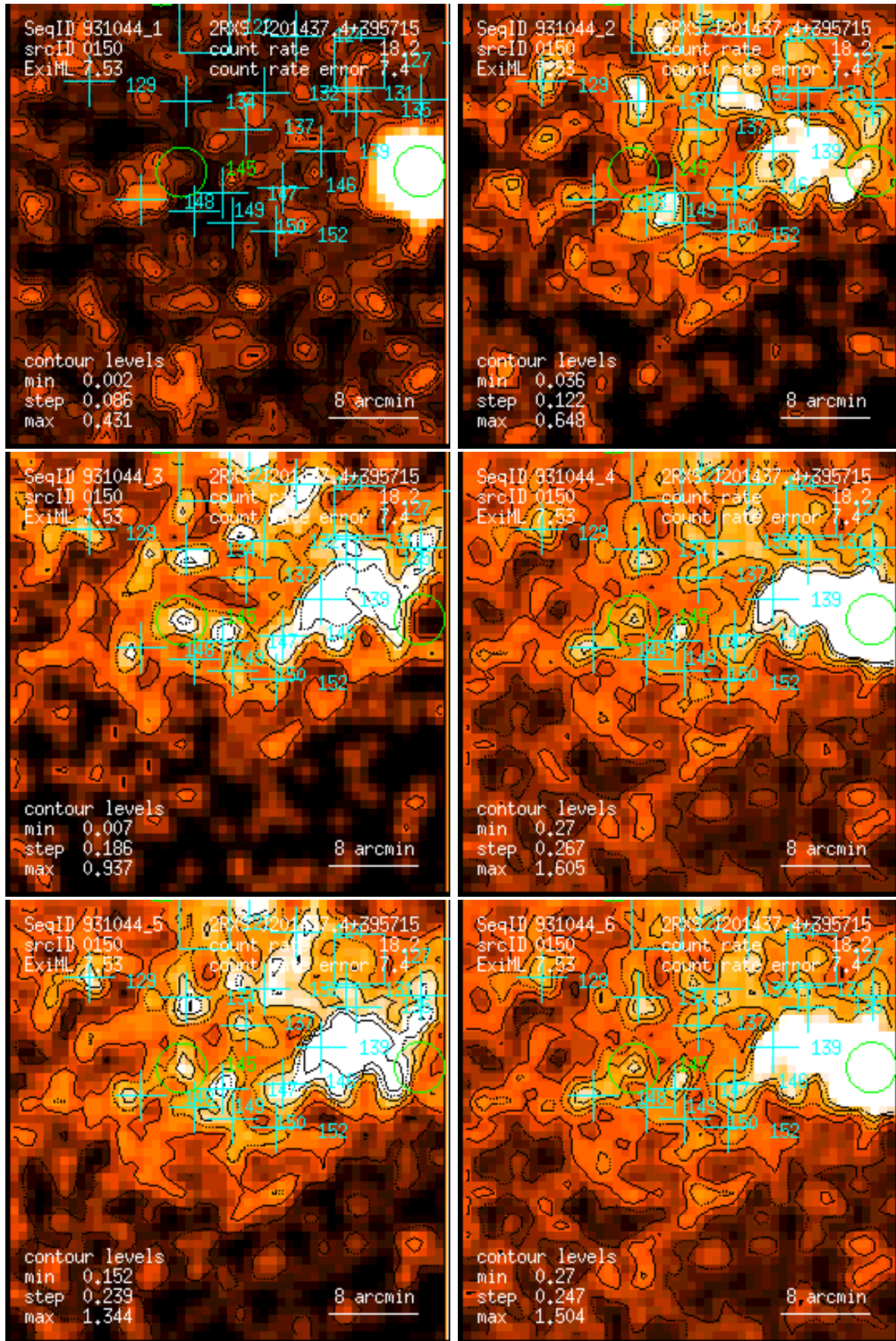
Figure 150: RASS 931044: detection 0150: band rate images, Gaussian filter: (1) PSPC channels 11 – 41, (2) 52 – 90, (3) 91 – 201, (4) 11 – 235, (5) 52 – 201, (6) 11 – 201. Broad band rates in counts/ks. Band rate contour levels in counts/ks/arcmin 2 .
