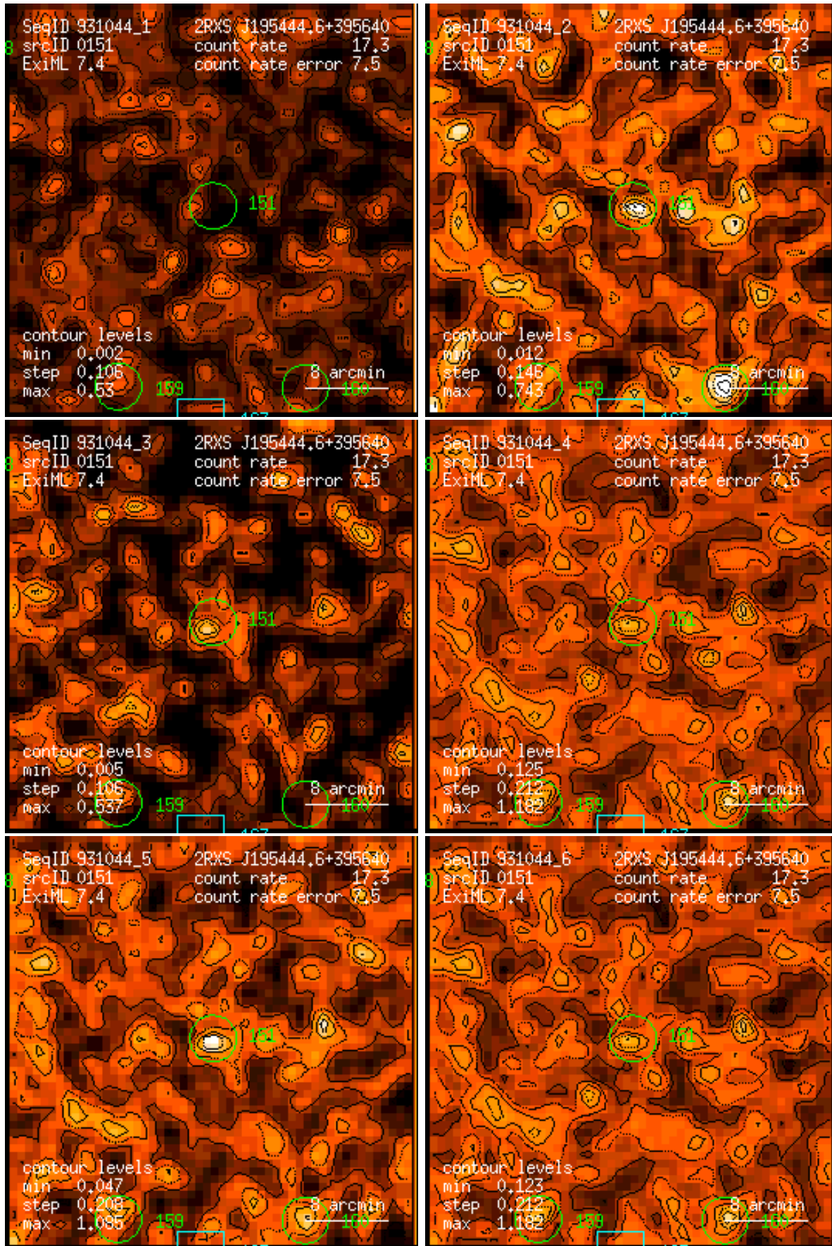
Figure 151: RASS 931044: detection 0151: band rate images, Gaussian filter: (1) PSPC channels 11 – 41, (2) 52 – 90, (3) 91 – 201, (4) 11 – 235, (5) 52 – 201, (6) 11 – 201. Broad band rates in counts/ks. Band rate contour levels in counts/ks/arcmin 2 .
