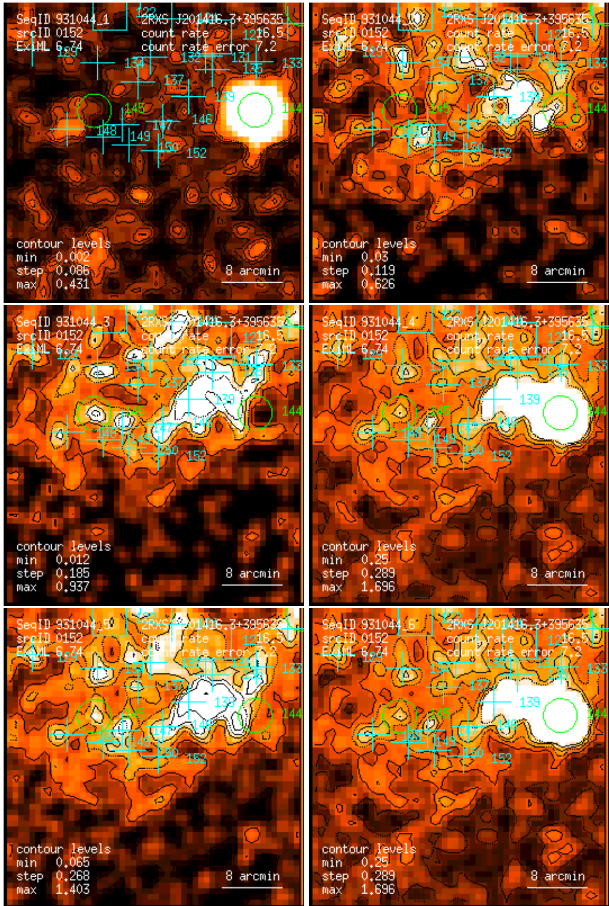
Figure 152: RASS 931044: detection 0152: band rate images, Gaussian filter: (1) PSPC channels 11 – 41, (2) 52 – 90, (3) 91 – 201, (4) 11 – 235, (5) 52 – 201, (6) 11 – 201. Broad band rates in counts/ks. Band rate contour levels in counts/ks/arcmin 2 .
