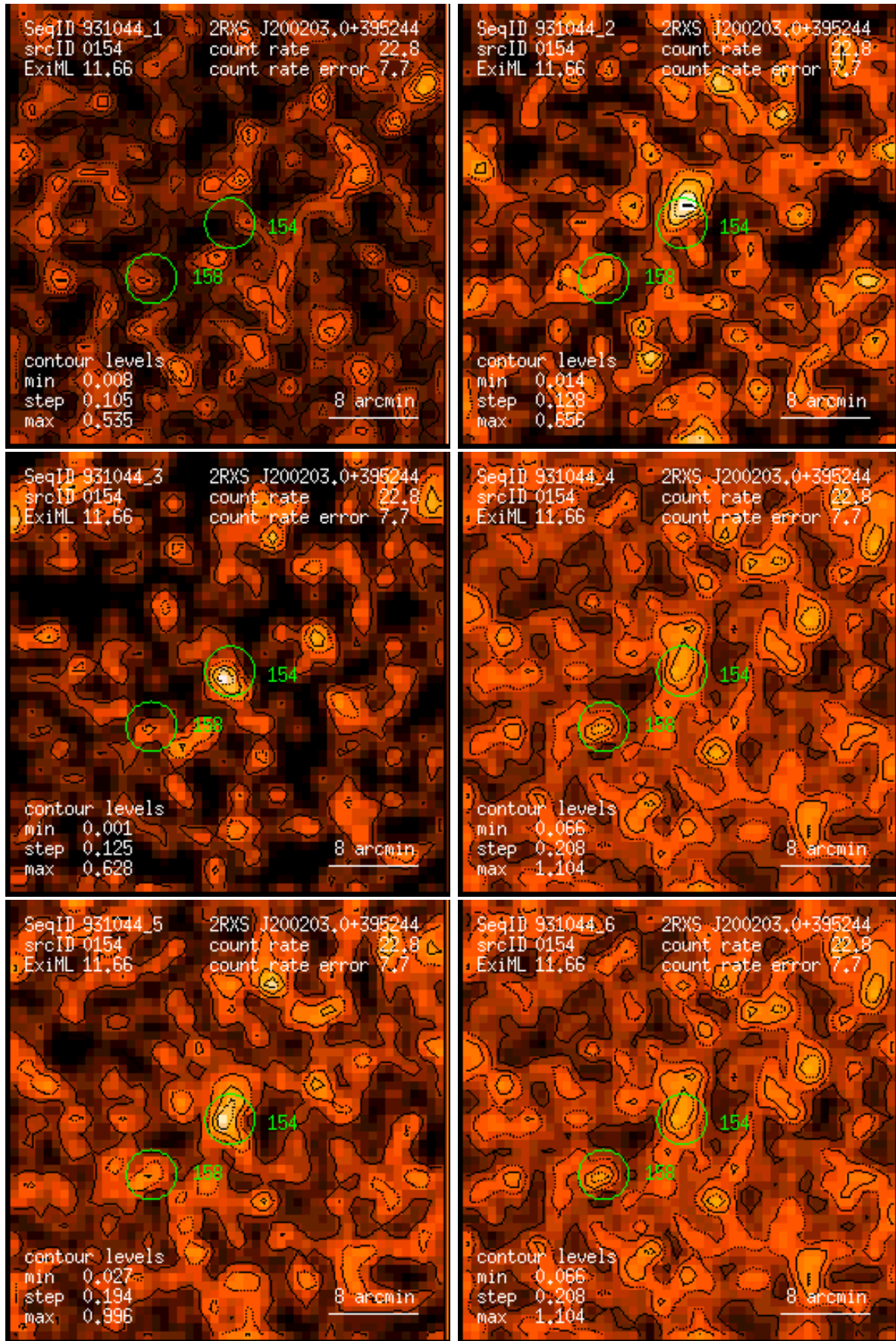
Figure 154: RASS 931044: detection 0154: band rate images, Gaussian filter: (1) PSPC channels 11 – 41, (2) 52 – 90, (3) 91 – 201, (4) 11 – 235, (5) 52 – 201, (6) 11 – 201. Broad band rates in counts/ks. Band rate contour levels in counts/ks/arcmin 2 .
