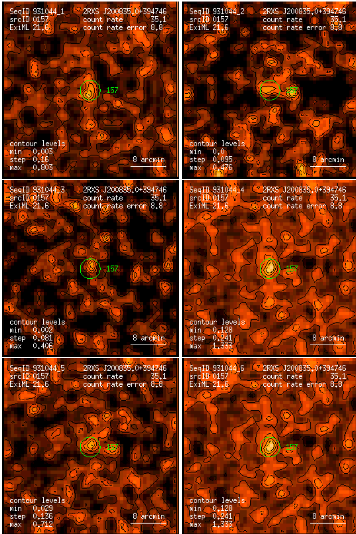
Figure 157: RASS 931044: detection 0157: band rate images, Gaussian filter: (1) PSPC channels 11 – 41, (2) 52 – 90, (3) 91 – 201, (4) 11 – 235, (5) 52 – 201, (6) 11 – 201. Broad band rates in counts/ks. Band rate contour levels in counts/ks/arcmin 2 .
