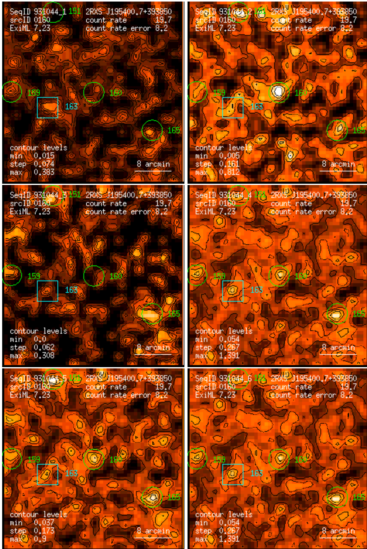
Figure 160: RASS 931044: detection 0160: band rate images, Gaussian filter: (1) PSPC channels 11 – 41, (2) 52 – 90, (3) 91 – 201, (4) 11 – 235, (5) 52 – 201, (6) 11 – 201. Broad band rates in counts/ks. Band rate contour levels in counts/ks/arcmin 2 .
