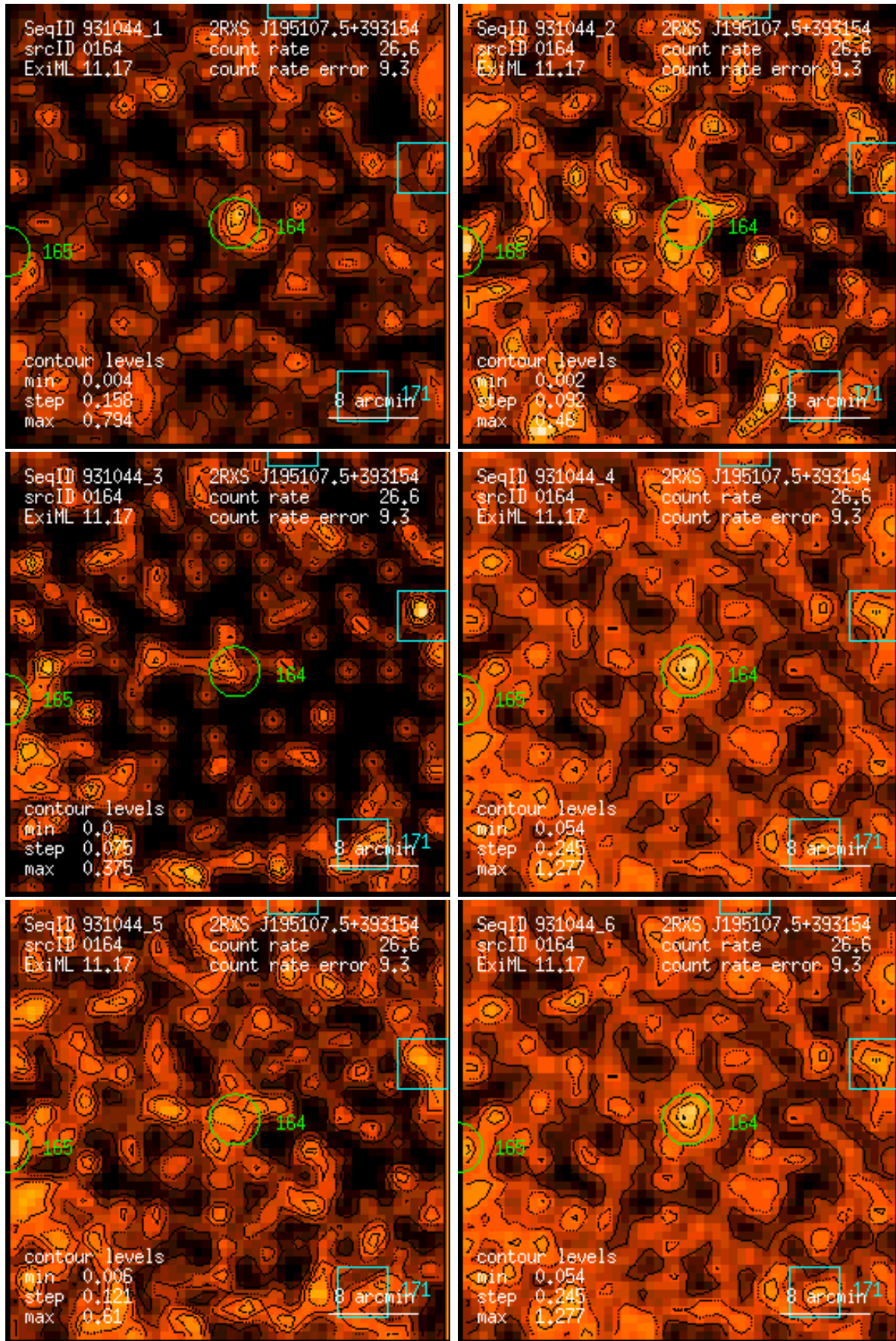
Figure 164: RASS 931044: detection 0164: band rate images, Gaussian filter: (1) PSPC channels 11 – 41, (2) 52 – 90, (3) 91 – 201, (4) 11 – 235, (5) 52 – 201, (6) 11 – 201. Broad band rates in counts/ks. Band rate contour levels in counts/ks/arcmin 2 .
