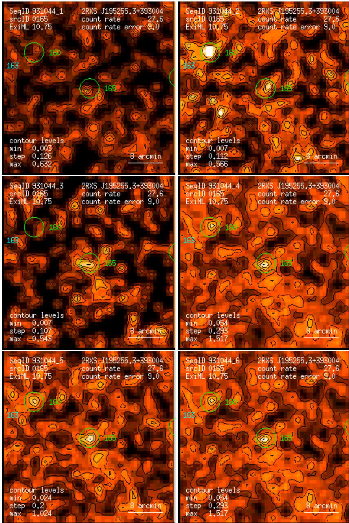
Figure 165: RASS 931044: detection 0165: band rate images, Gaussian filter: (1) PSPC channels 11 – 41, (2) 52 – 90, (3) 91 – 201, (4) 11 – 235, (5) 52 – 201, (6) 11 – 201. Broad band rates in counts/ks. Band rate contour levels in counts/ks/arcmin 2 .
