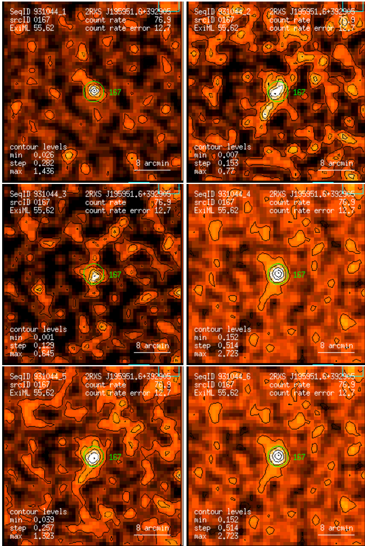
Figure 167: RASS 931044: detection 0167: band rate images, Gaussian filter: (1) PSPC channels 11 – 41, (2) 52 – 90, (3) 91 – 201, (4) 11 – 235, (5) 52 – 201, (6) 11 – 201. Broad band rates in counts/ks. Band rate contour levels in counts/ks/arcmin 2 .
