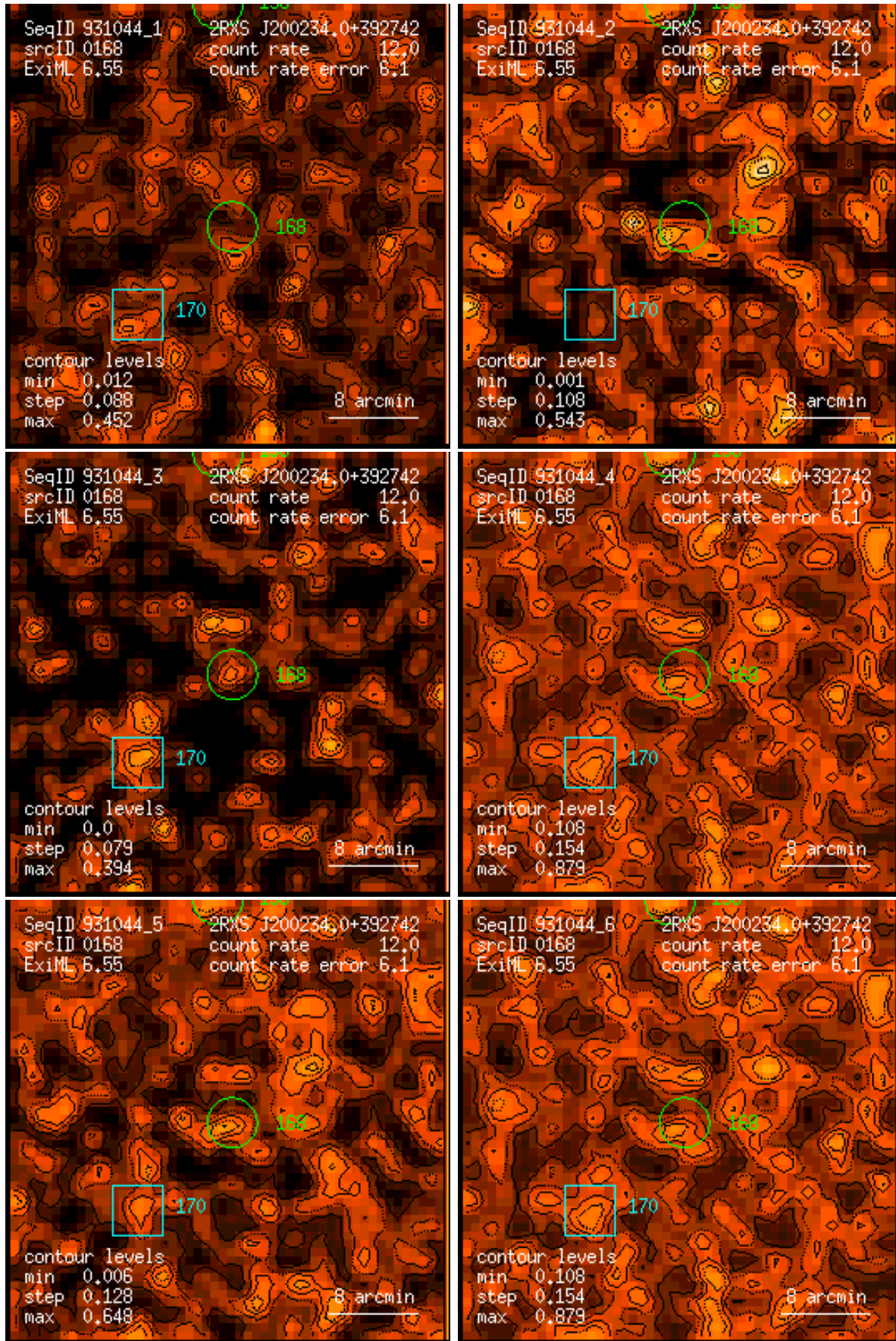
Figure 168: RASS 931044: detection 0168: band rate images, Gaussian filter: (1) PSPC channels 11 – 41, (2) 52 – 90, (3) 91 – 201, (4) 11 – 235, (5) 52 – 201, (6) 11 – 201. Broad band rates in counts/ks. Band rate contour levels in counts/ks/arcmin 2 .
