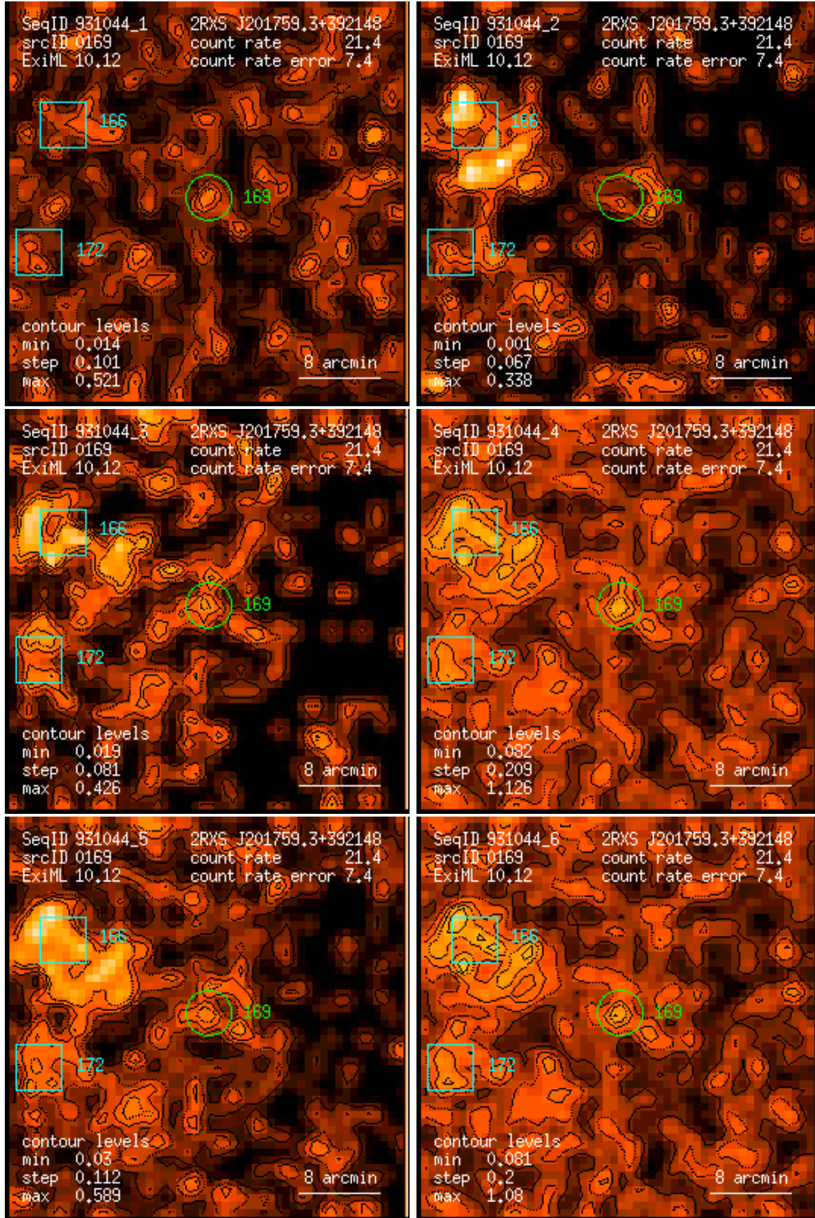
Figure 169: RASS 931044: detection 0169: band rate images, Gaussian filter: (1) PSPC channels 11 – 41, (2) 52 – 90, (3) 91 – 201, (4) 11 – 235, (5) 52 – 201, (6) 11 – 201. Broad band rates in counts/ks. Band rate contour levels in counts/ks/arcmin 2 .
