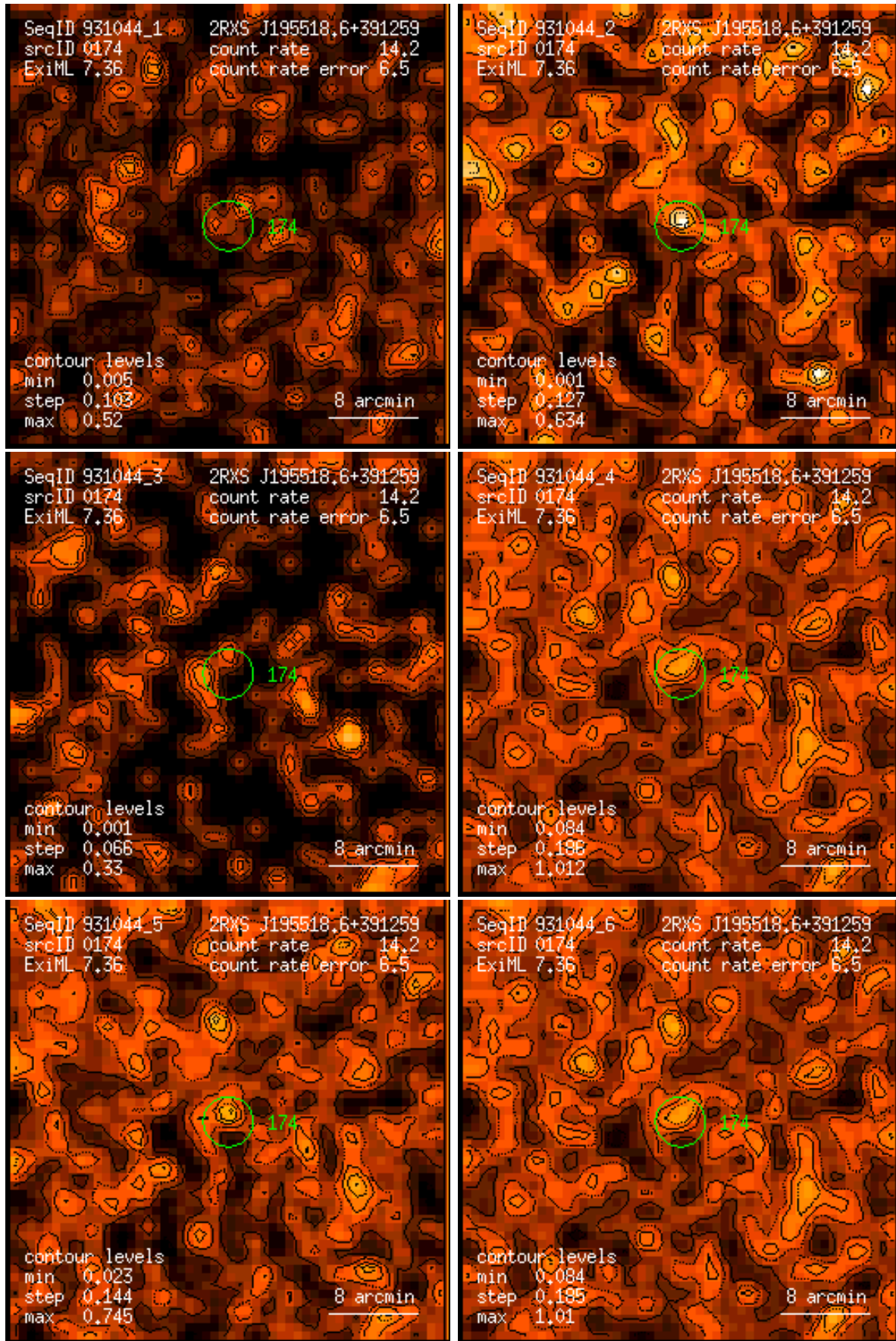
Figure 174: RASS 931044: detection 0174: band rate images, Gaussian filter: (1) PSPC channels 11 – 41, (2) 52 – 90, (3) 91 – 201, (4) 11 – 235, (5) 52 – 201, (6) 11 – 201. Broad band rates in counts/ks. Band rate contour levels in counts/ks/arcmin 2 .
