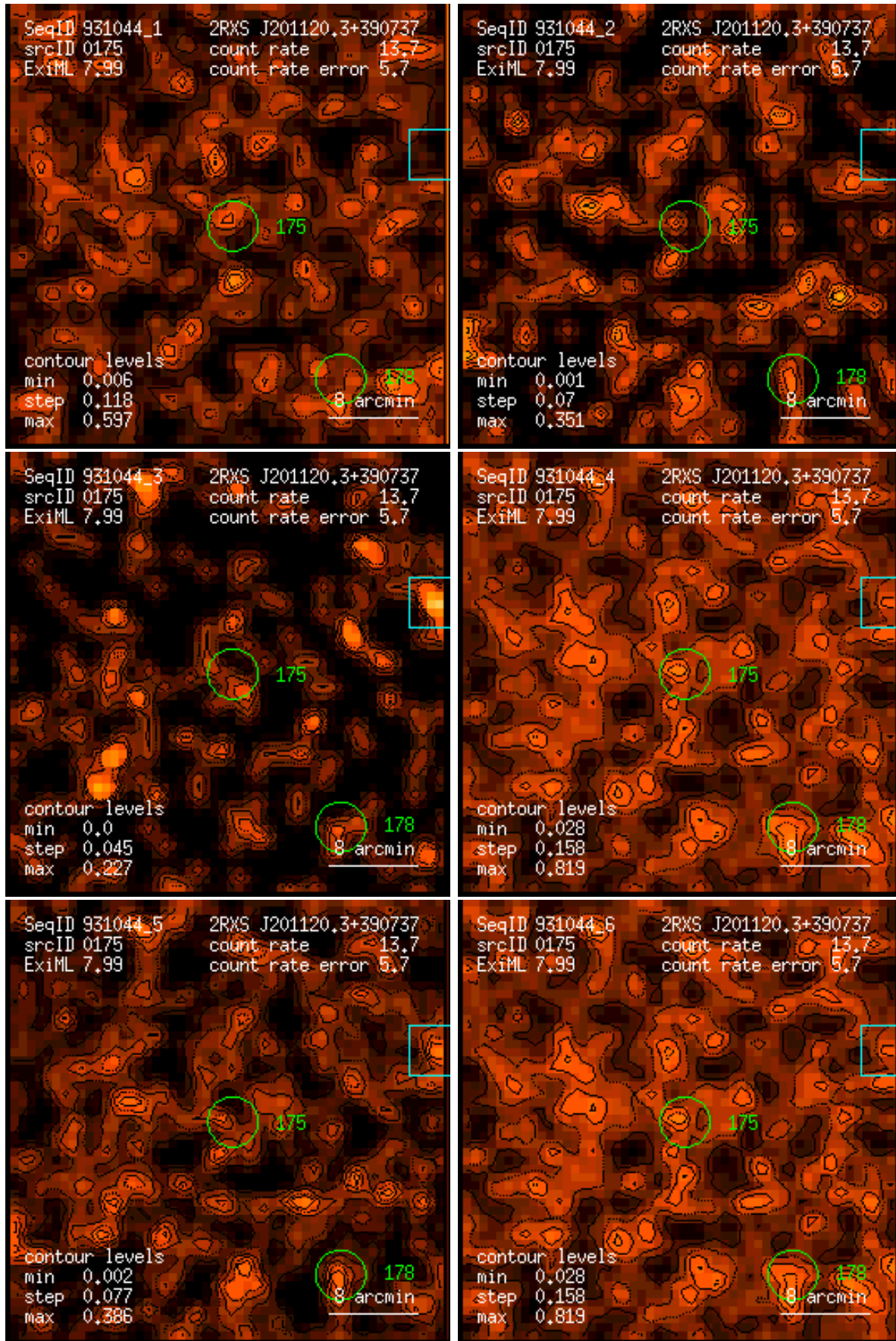
Figure 175: RASS 931044: detection 0175: band rate images, Gaussian filter: (1) PSPC channels 11 – 41, (2) 52 – 90, (3) 91 – 201, (4) 11 – 235, (5) 52 – 201, (6) 11 – 201. Broad band rates in counts/ks. Band rate contour levels in counts/ks/arcmin 2 .
