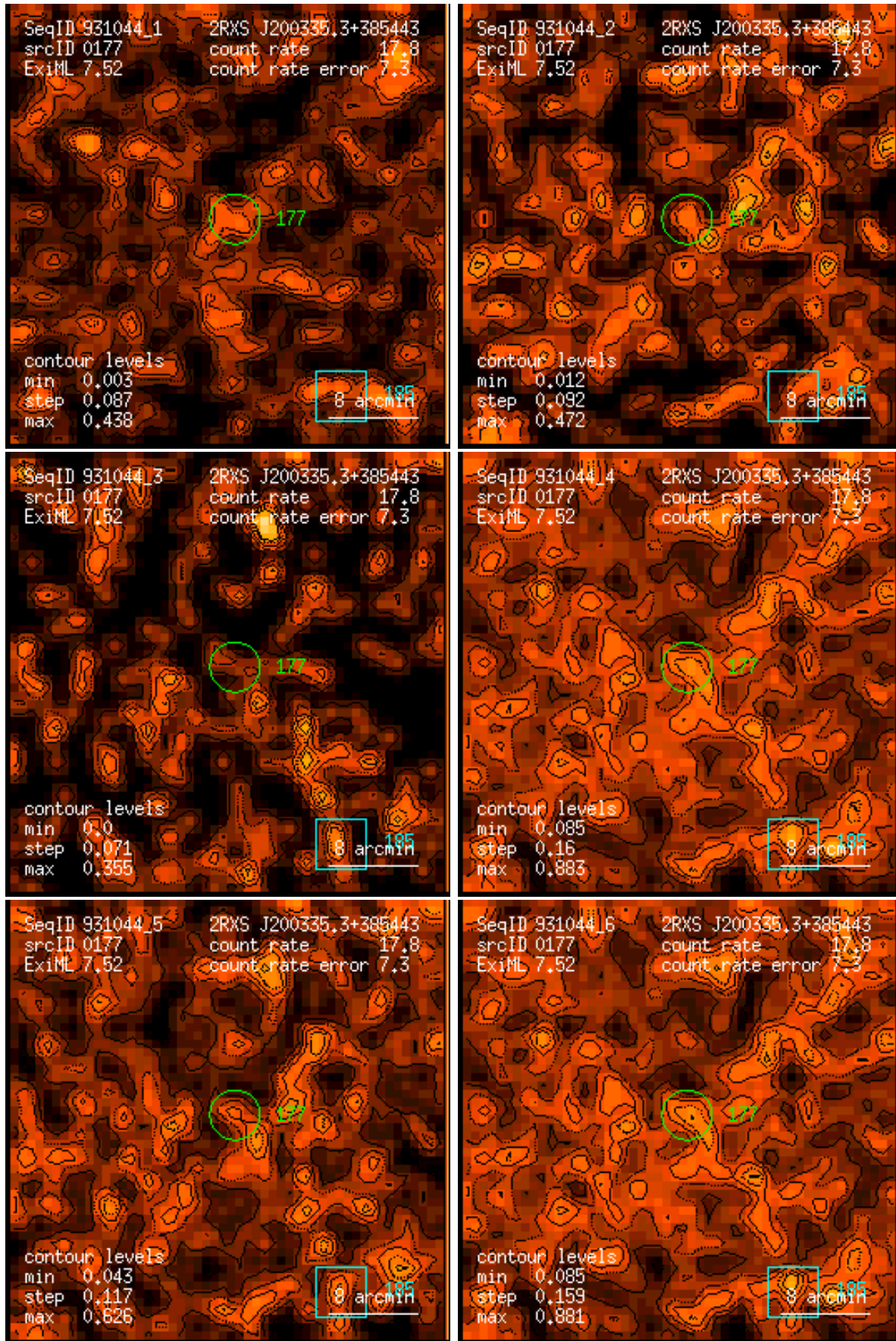
Figure 177: RASS 931044: detection 0177: band rate images, Gaussian filter: (1) PSPC channels 11 – 41, (2) 52 – 90, (3) 91 – 201, (4) 11 – 235, (5) 52 – 201, (6) 11 – 201. Broad band rates in counts/ks. Band rate contour levels in counts/ks/arcmin 2 .
