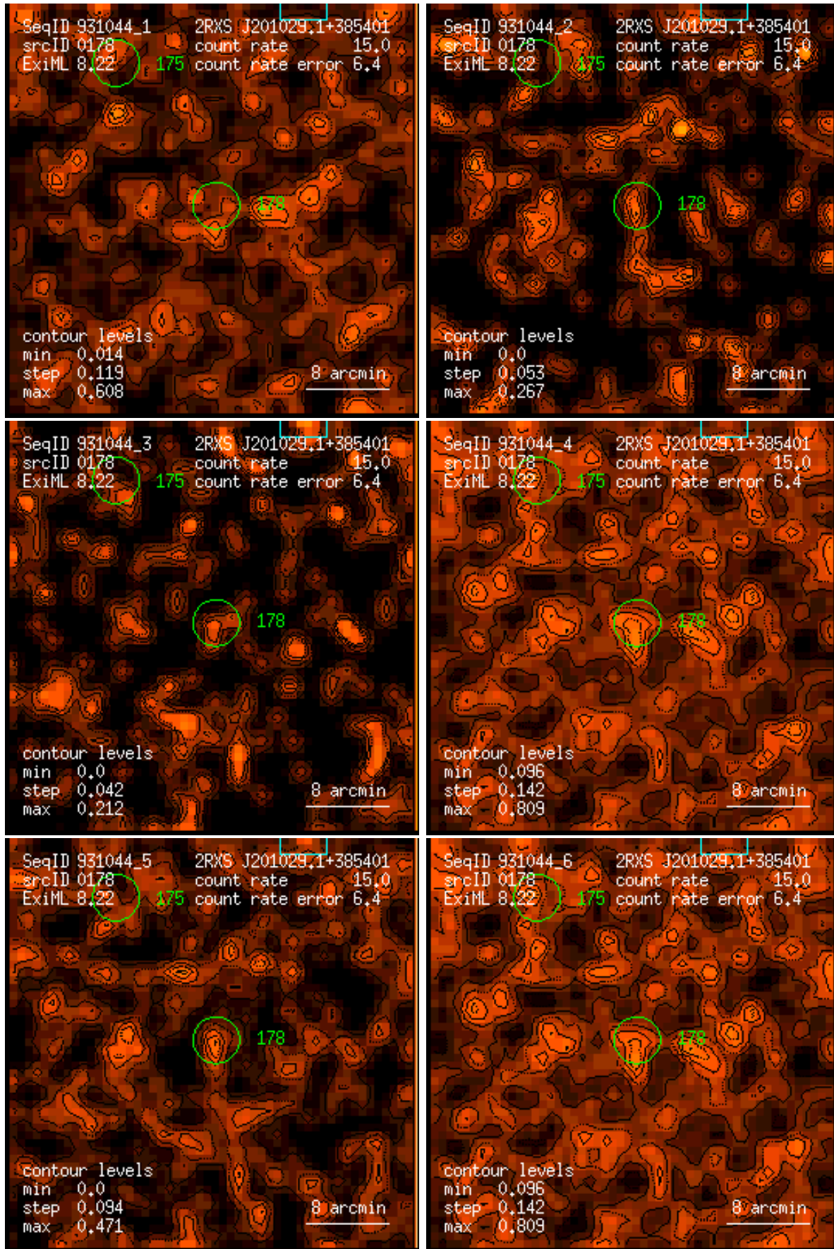
Figure 178: RASS 931044: detection 0178: band rate images, Gaussian filter: (1) PSPC channels 11 – 41, (2) 52 – 90, (3) 91 – 201, (4) 11 – 235, (5) 52 – 201, (6) 11 – 201. Broad band rates in counts/ks. Band rate contour levels in counts/ks/arcmin 2 .
