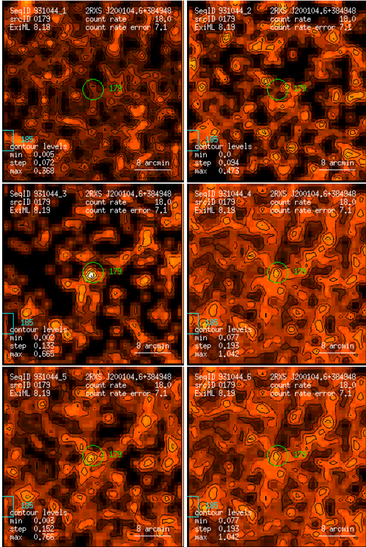
Figure 179: RASS 931044: detection 0179: band rate images, Gaussian filter: (1) PSPC channels 11 – 41, (2) 52 – 90, (3) 91 – 201, (4) 11 – 235, (5) 52 – 201, (6) 11 – 201. Broad band rates in counts/ks. Band rate contour levels in counts/ks/arcmin 2 .
