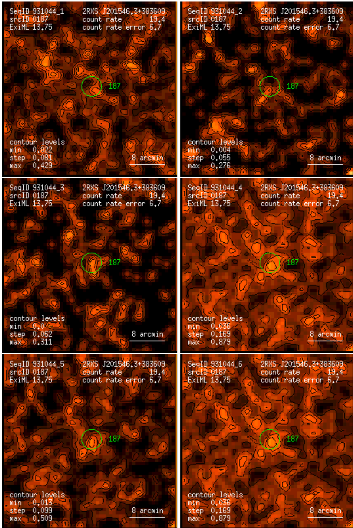
Figure 187: RASS 931044: detection 0187: band rate images, Gaussian filter: (1) PSPC channels 11 – 41, (2) 52 – 90, (3) 91 – 201, (4) 11 – 235, (5) 52 – 201, (6) 11 – 201. Broad band rates in counts/ks. Band rate contour levels in counts/ks/arcmin 2 .
