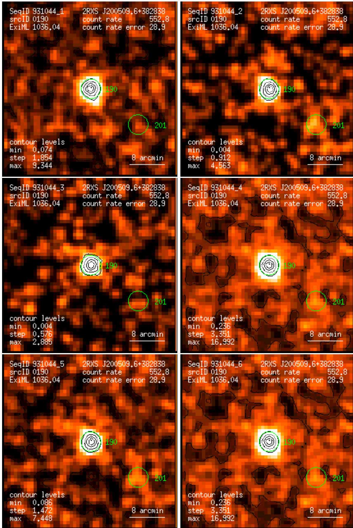
Figure 190: RASS 931044: detection 0190: band rate images, Gaussian filter: (1) PSPC channels 11 – 41, (2) 52 – 90, (3) 91 – 201, (4) 11 – 235, (5) 52 – 201, (6) 11 – 201. Broad band rates in counts/ks. Band rate contour levels in counts/ks/arcmin 2 .
