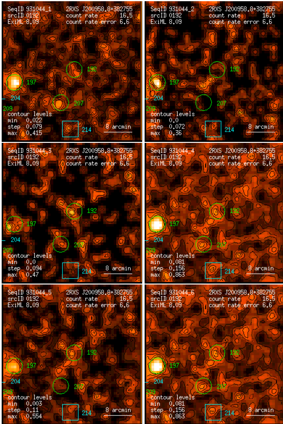
Figure 192: RASS 931044: detection 0192: band rate images, Gaussian filter: (1) PSPC channels 11 – 41, (2) 52 – 90, (3) 91 – 201, (4) 11 – 235, (5) 52 – 201, (6) 11 – 201. Broad band rates in counts/ks. Band rate contour levels in counts/ks/arcmin 2 .
