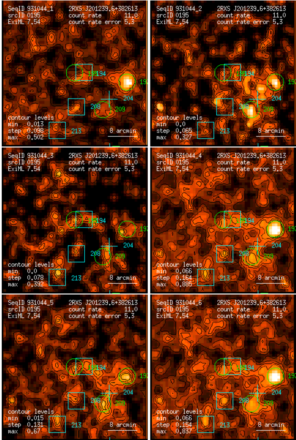
Figure 195: RASS 931044: detection 0195: band rate images, Gaussian filter: (1) PSPC channels 11 – 41, (2) 52 – 90, (3) 91 – 201, (4) 11 – 235, (5) 52 – 201, (6) 11 – 201. Broad band rates in counts/ks. Band rate contour levels in counts/ks/arcmin 2 .
