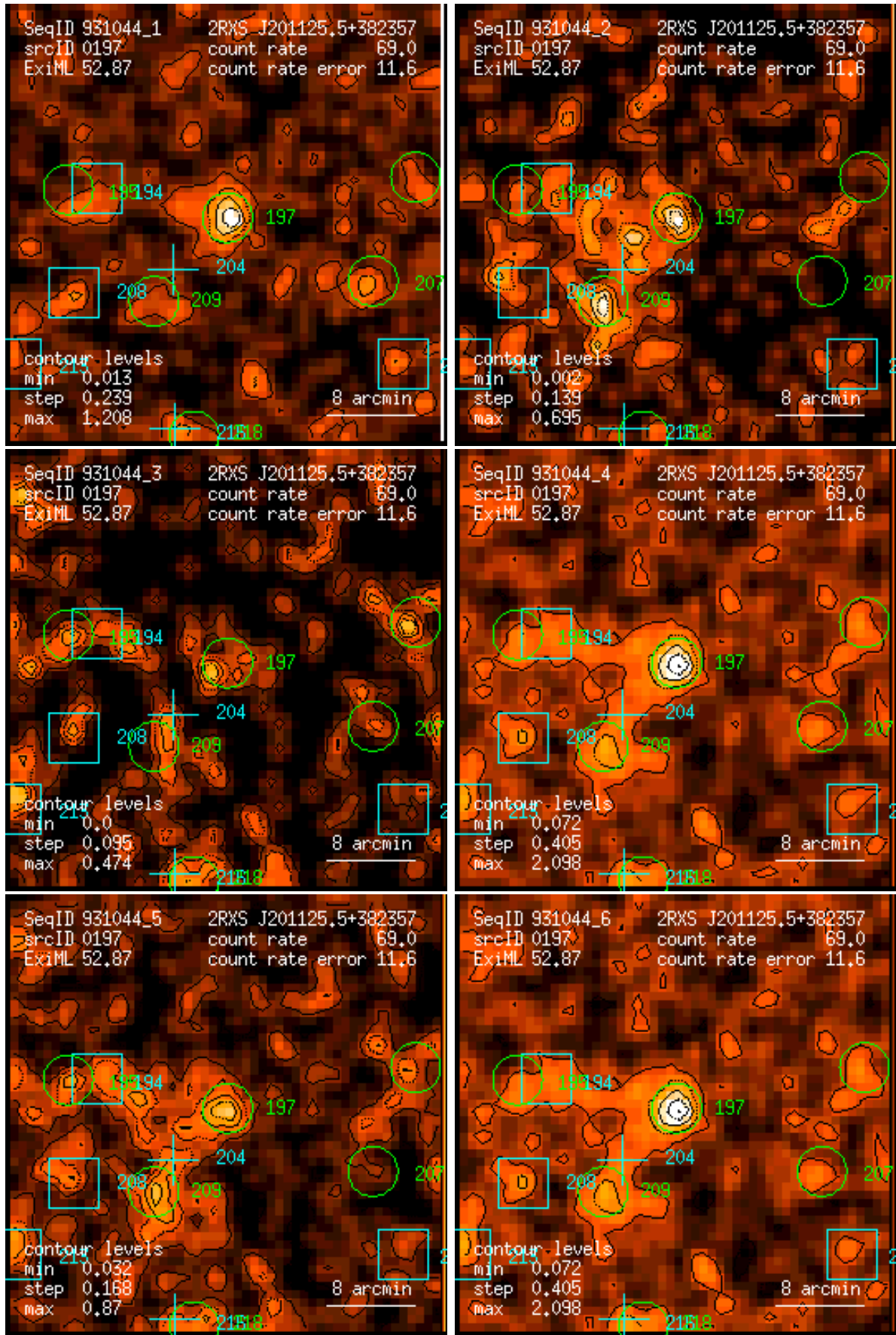
Figure 197: RASS 931044: detection 0197: band rate images, Gaussian filter: (1) PSPC channels 11 – 41, (2) 52 – 90, (3) 91 – 201, (4) 11 – 235, (5) 52 – 201, (6) 11 – 201. Broad band rates in counts/ks. Band rate contour levels in counts/ks/arcmin 2 .
