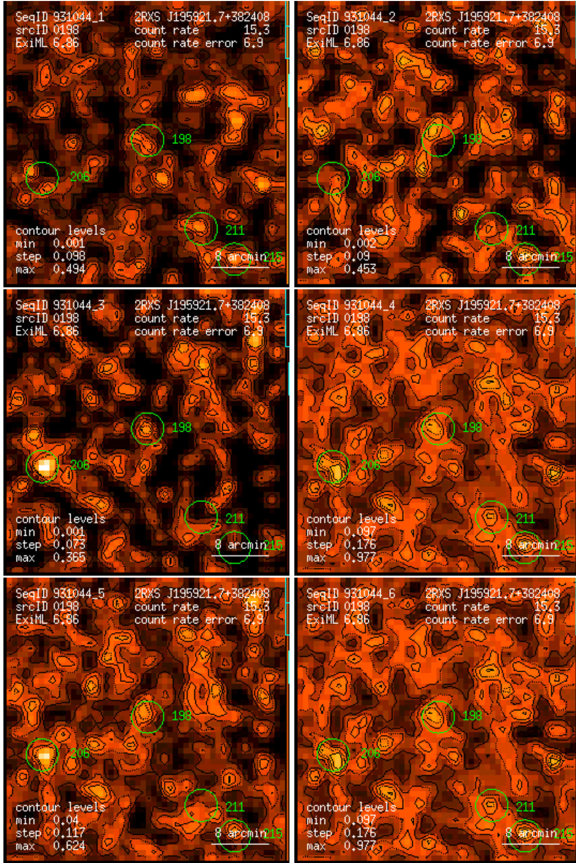
Figure 198: RASS 931044: detection 0198: band rate images, Gaussian filter: (1) PSPC channels 11 – 41, (2) 52 – 90, (3) 91 – 201, (4) 11 – 235, (5) 52 – 201, (6) 11 – 201. Broad band rates in counts/ks. Band rate contour levels in counts/ks/arcmin 2 .
