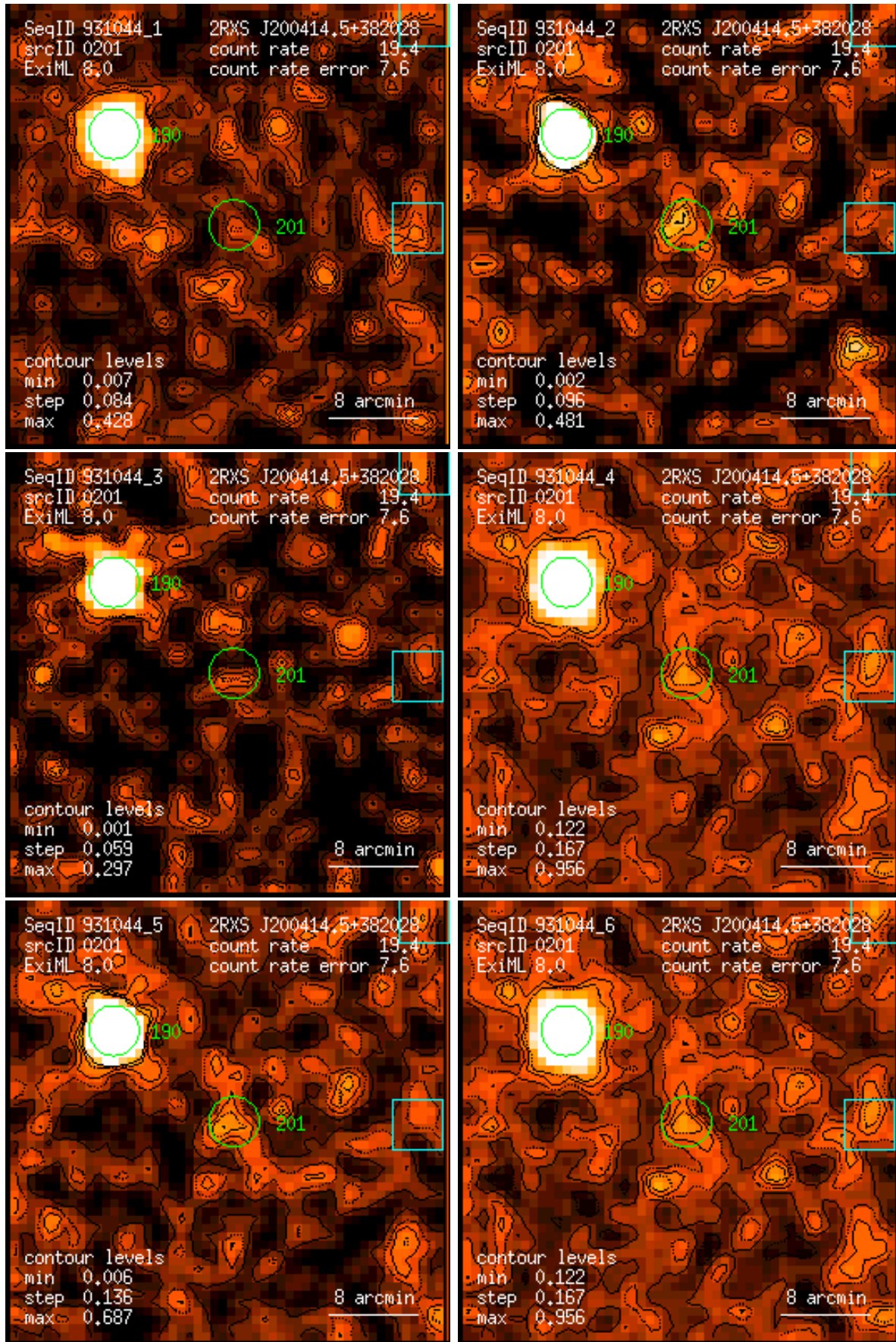
Figure 201: RASS 931044: detection 0201: band rate images, Gaussian filter: (1) PSPC channels 11 – 41, (2) 52 – 90, (3) 91 – 201, (4) 11 – 235, (5) 52 – 201, (6) 11 – 201. Broad band rates in counts/ks. Band rate contour levels in counts/ks/arcmin 2 .
