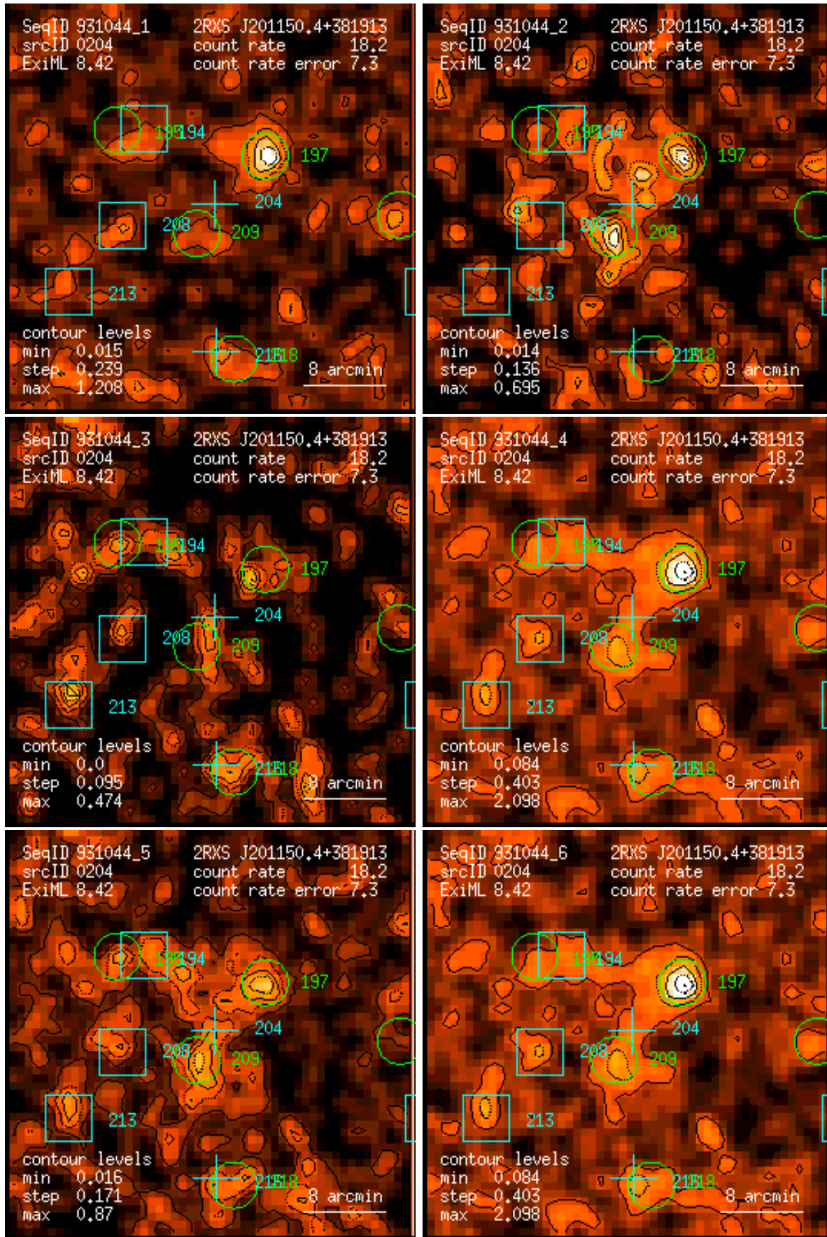
Figure 204: RASS 931044: detection 0204: band rate images, Gaussian filter: (1) PSPC channels 11 – 41, (2) 52 – 90, (3) 91 – 201, (4) 11 – 235, (5) 52 – 201, (6) 11 – 201. Broad band rates in counts/ks. Band rate contour levels in counts/ks/arcmin 2 .
