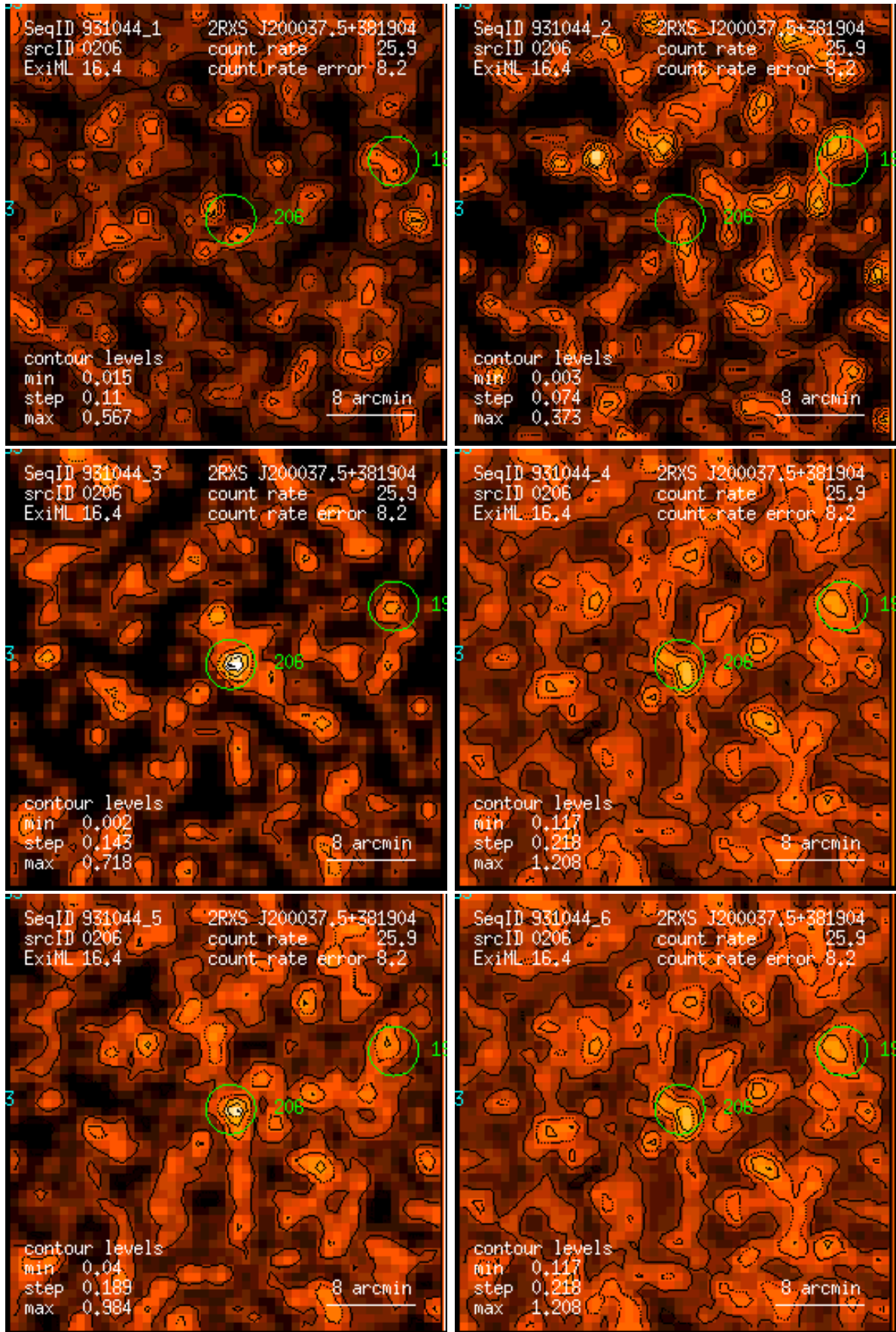
Figure 206: RASS 931044: detection 0206: band rate images, Gaussian filter: (1) PSPC channels 11 – 41, (2) 52 – 90, (3) 91 – 201, (4) 11 – 235, (5) 52 – 201, (6) 11 – 201. Broad band rates in counts/ks. Band rate contour levels in counts/ks/arcmin 2 .
