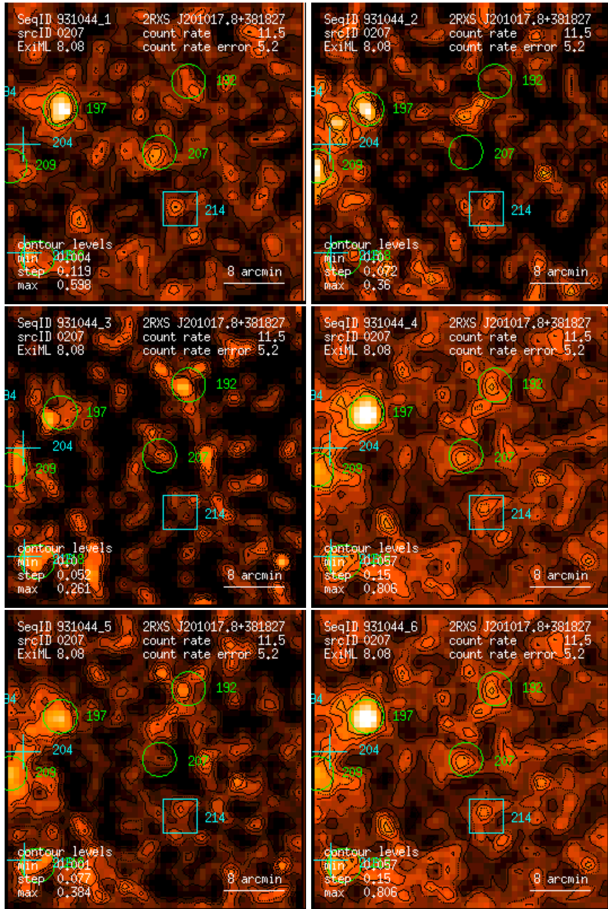
Figure 207: RASS 931044: detection 0207: band rate images, Gaussian filter: (1) PSPC channels 11 – 41, (2) 52 – 90, (3) 91 – 201, (4) 11 – 235, (5) 52 – 201, (6) 11 – 201. Broad band rates in counts/ks. Band rate contour levels in counts/ks/arcmin 2 .
