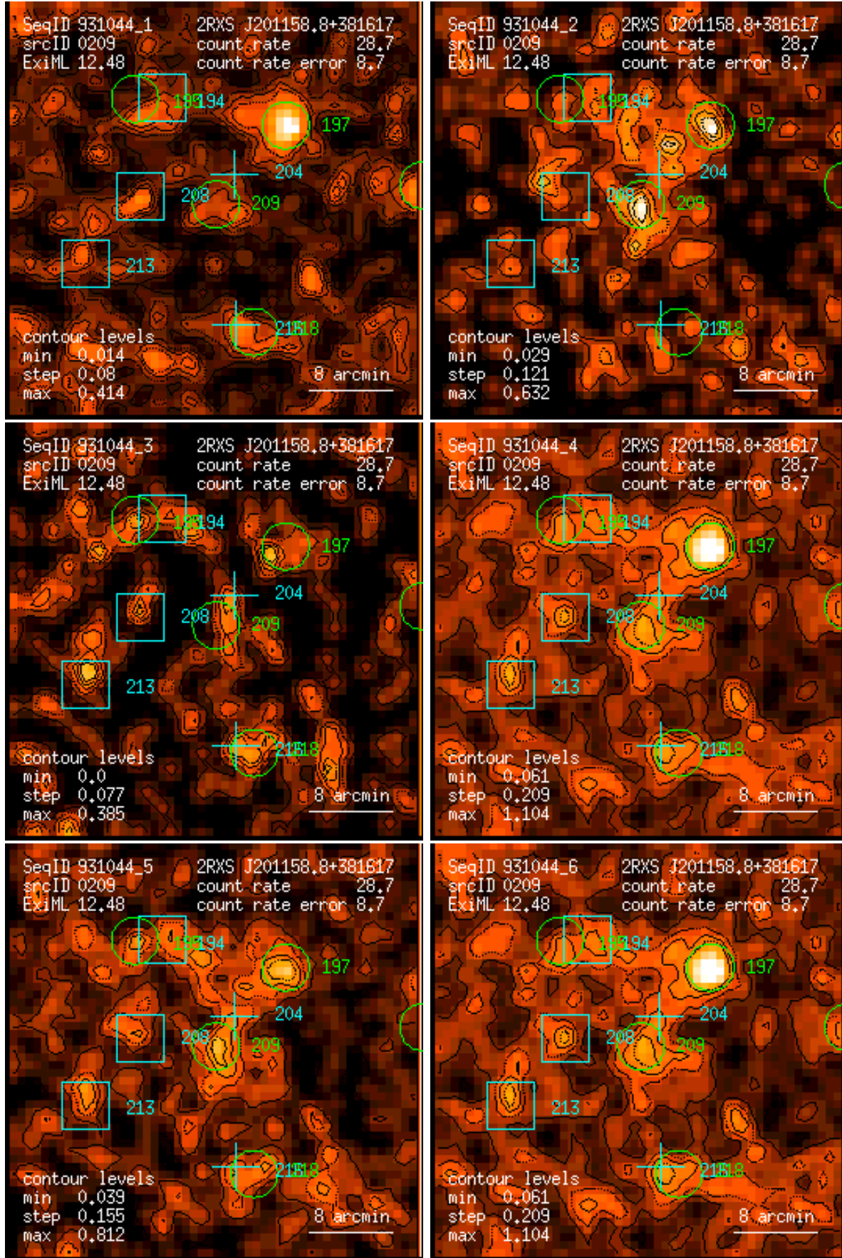
Figure 209: RASS 931044: detection 0209: band rate images, Gaussian filter: (1) PSPC channels 11 – 41, (2) 52 – 90, (3) 91 – 201, (4) 11 – 235, (5) 52 – 201, (6) 11 – 201. Broad band rates in counts/ks. Band rate contour levels in counts/ks/arcmin 2 .
