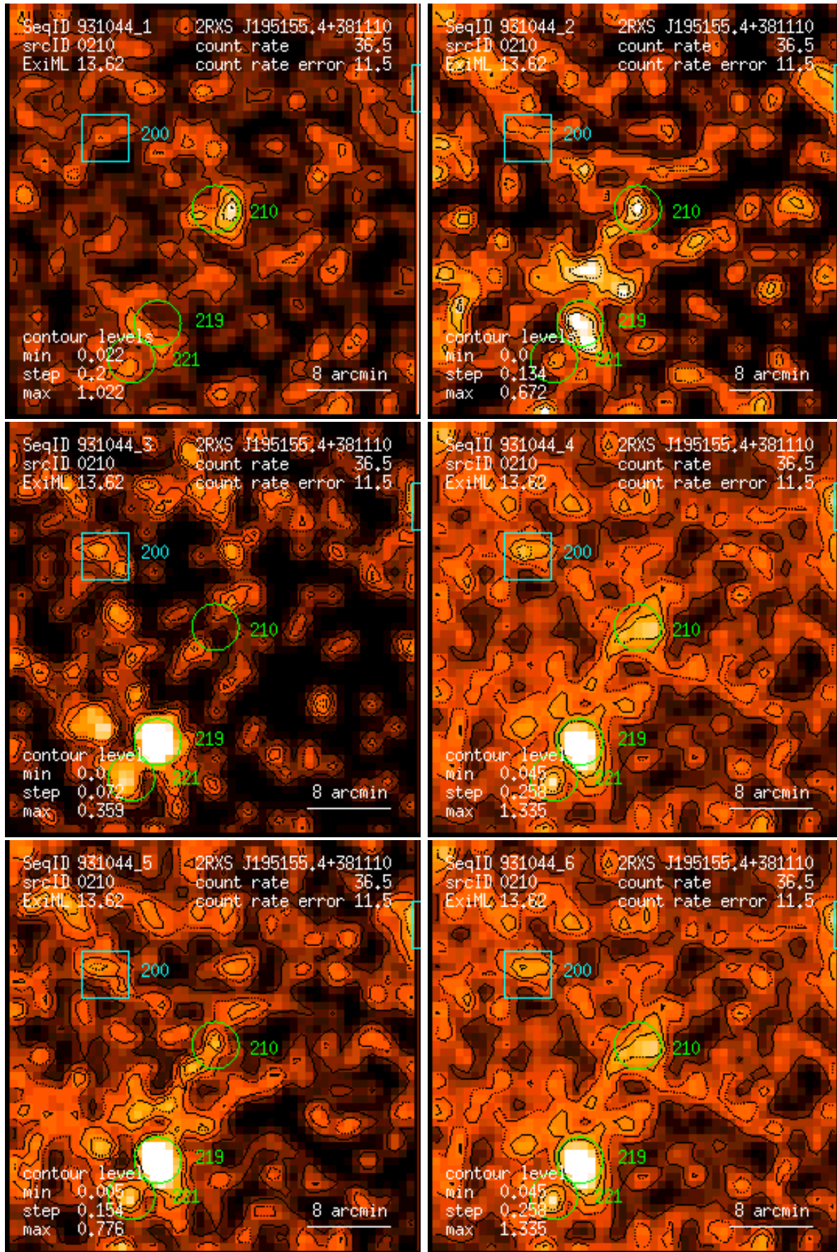
Figure 210: RASS 931044: detection 0210: band rate images, Gaussian filter: (1) PSPC channels 11 – 41, (2) 52 – 90, (3) 91 – 201, (4) 11 – 235, (5) 52 – 201, (6) 11 – 201. Broad band rates in counts/ks. Band rate contour levels in counts/ks/arcmin 2 .
