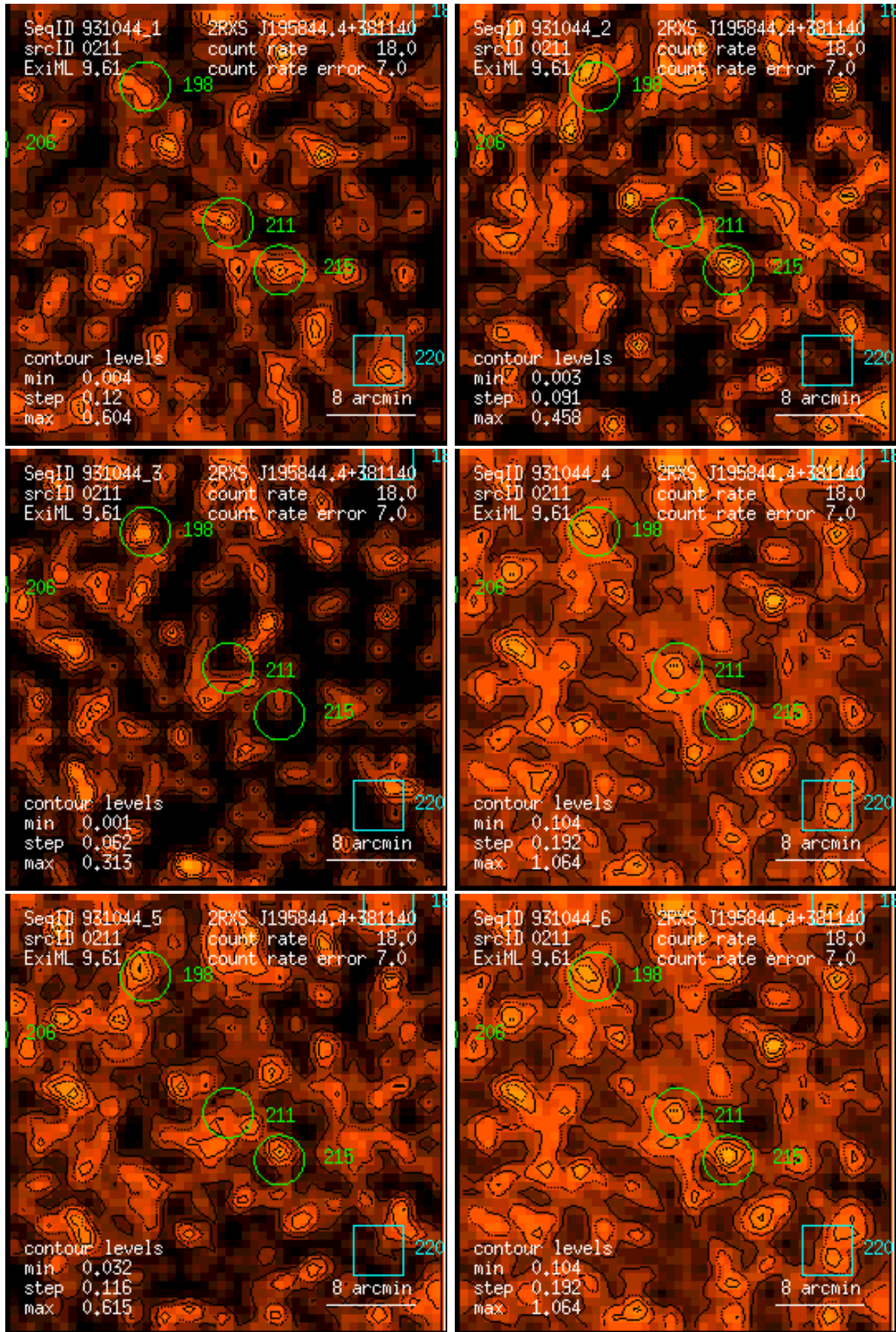
Figure 211: RASS 931044: detection 0211: band rate images, Gaussian filter: (1) PSPC channels 11 – 41, (2) 52 – 90, (3) 91 – 201, (4) 11 – 235, (5) 52 – 201, (6) 11 – 201. Broad band rates in counts/ks. Band rate contour levels in counts/ks/arcmin 2 .
