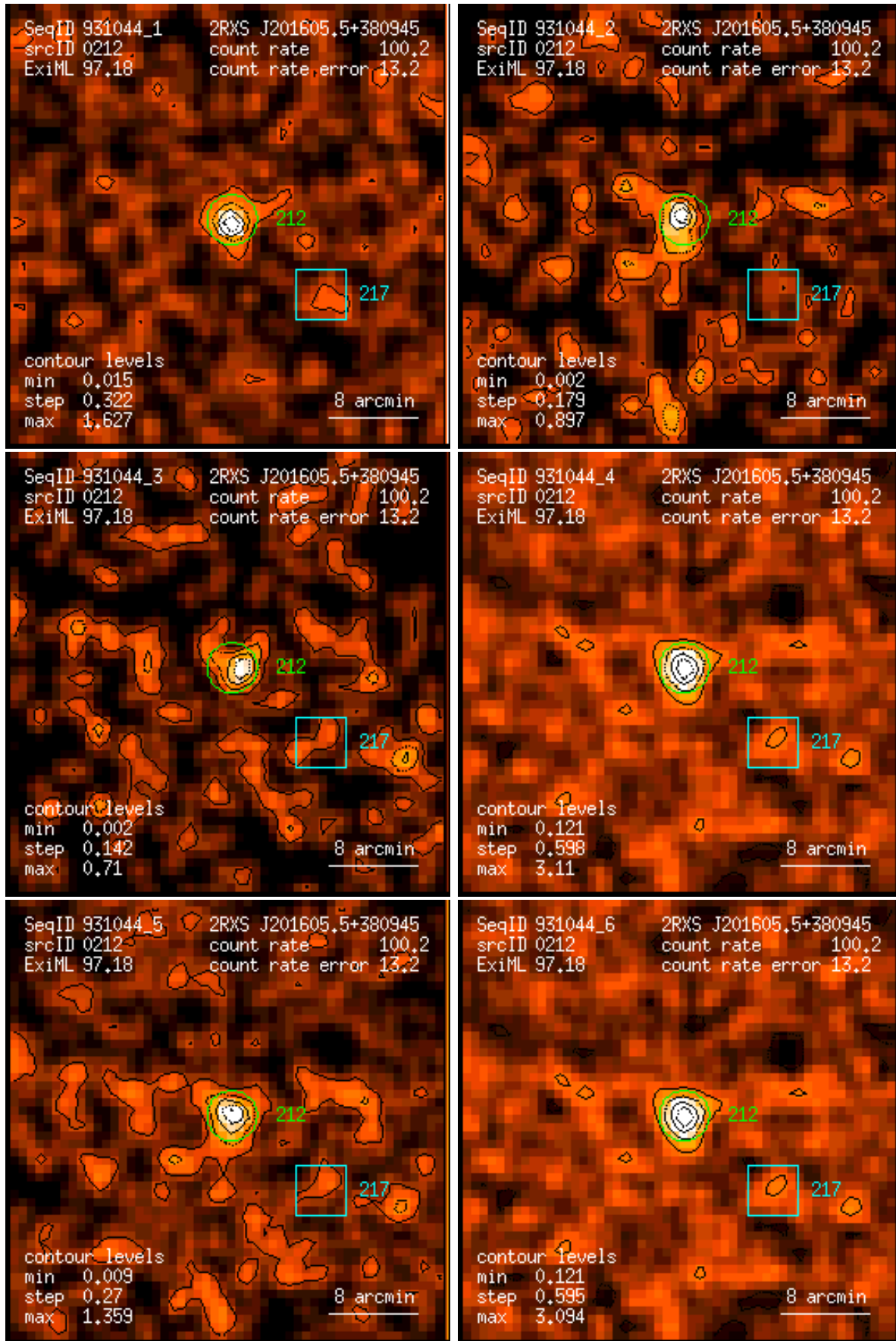
Figure 212: RASS 931044: detection 0212: band rate images, Gaussian filter: (1) PSPC channels 11 – 41, (2) 52 – 90, (3) 91 – 201, (4) 11 – 235, (5) 52 – 201, (6) 11 – 201. Broad band rates in counts/ks. Band rate contour levels in counts/ks/arcmin 2 .
